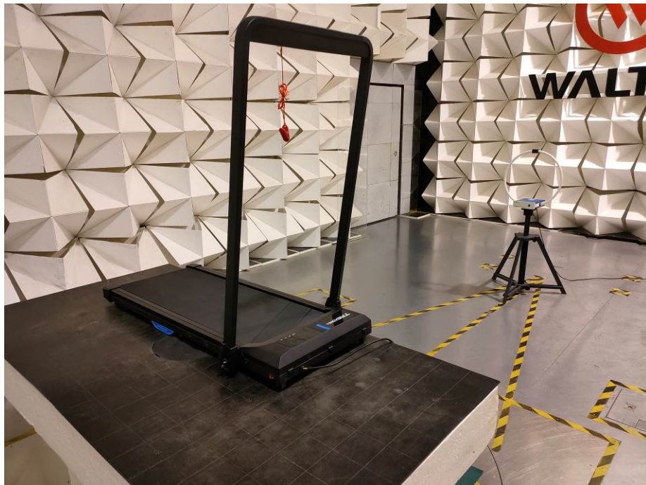
Model T38 For 9kHz-30MHz Test Site 2#
