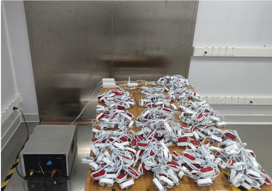
Photos of Conducted Emission Test
