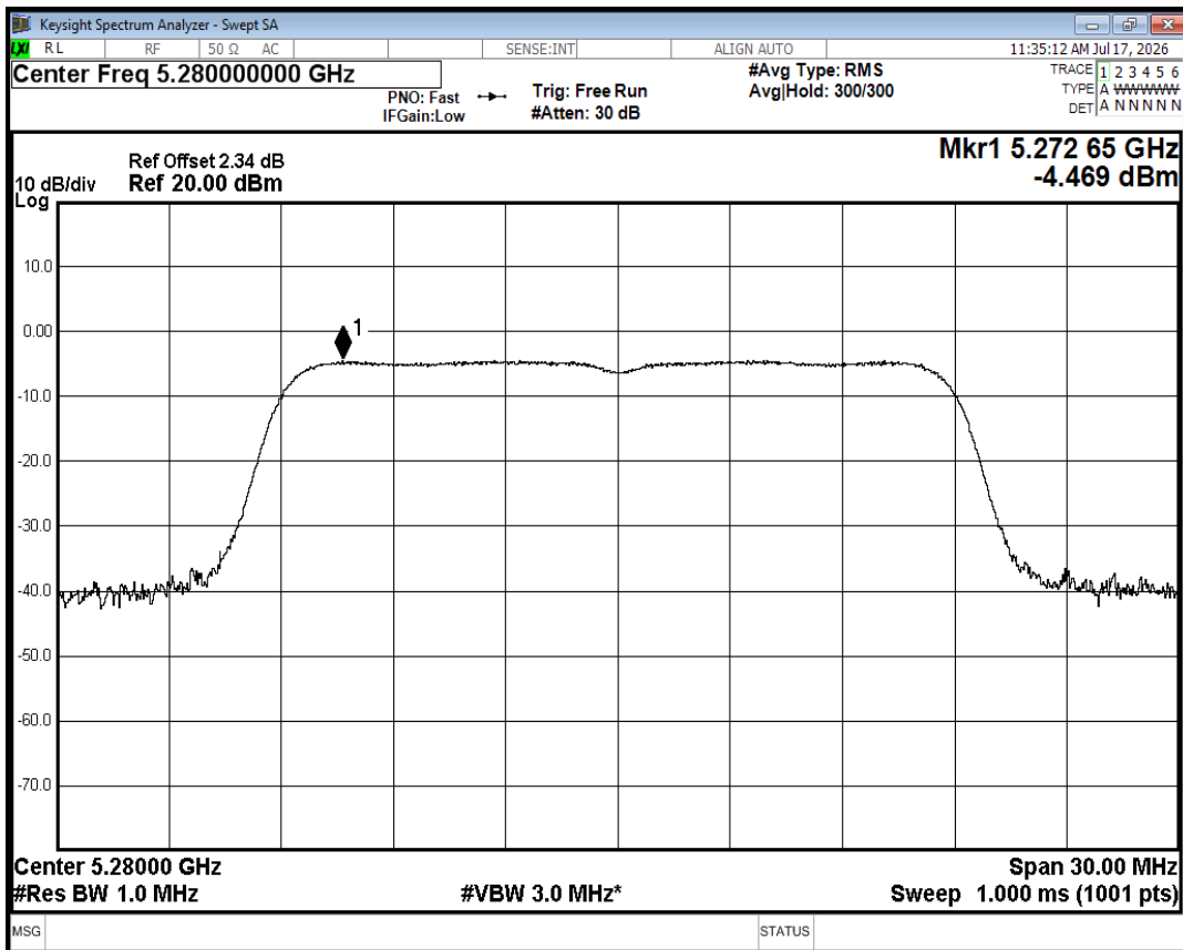
PSD NVNT n20 5280MHz Ant1
