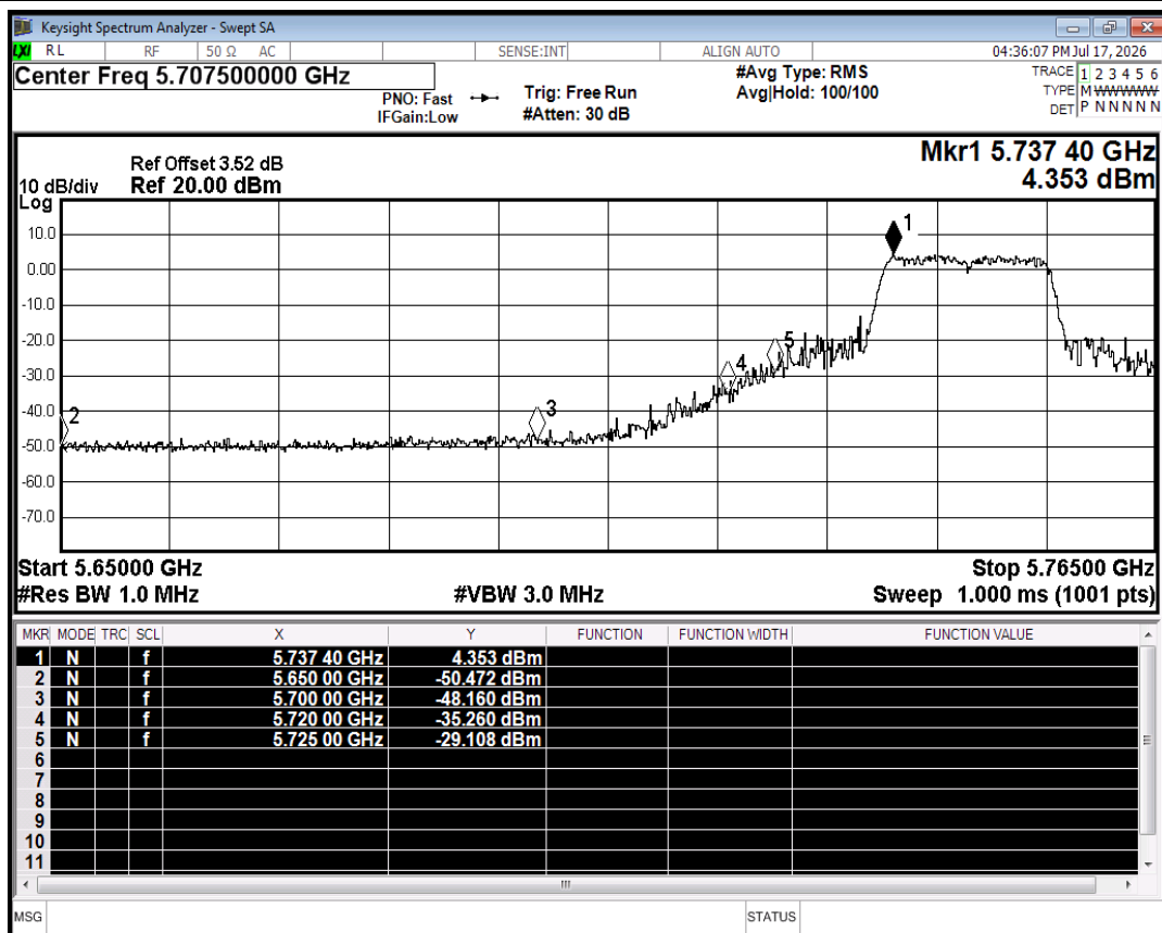
Restrict Band NVNT n20 5745MHz Ant1 Peak
