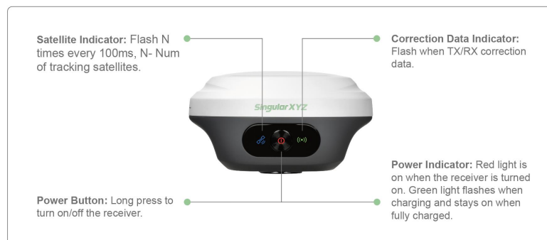
Front Panel
