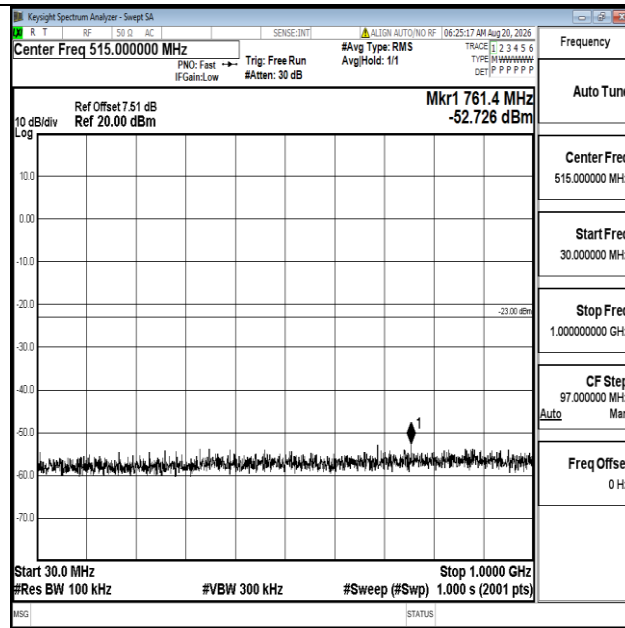
Band4-20MHz-QPSK-20050-1RB#0-30~1000-PASS
