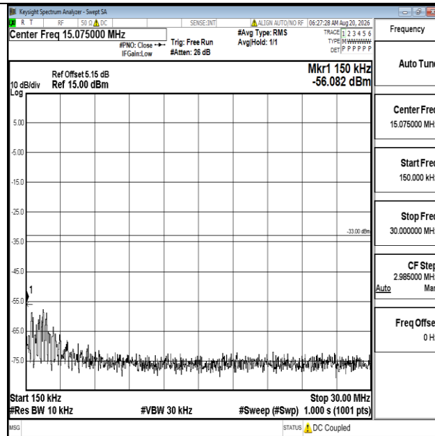
Band4-20MHz-16QAM-20175-1RB#0-0.15~30-PASS
