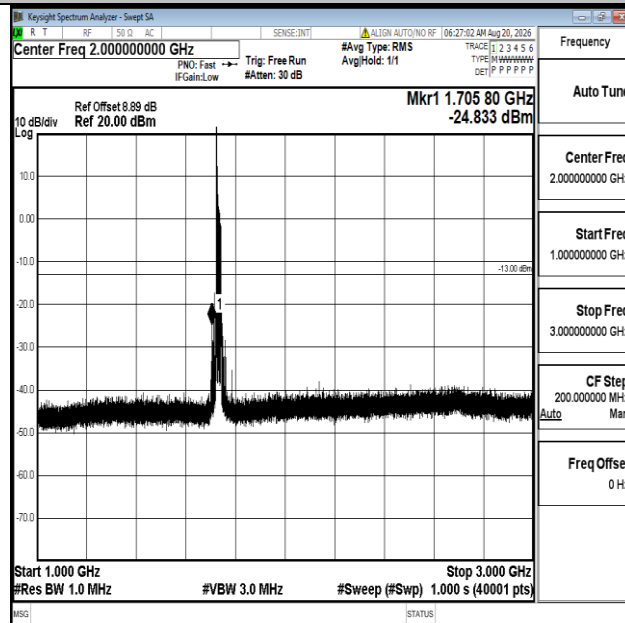
Band4-20MHz-QPSK-20175-1RB#0-1000~3000-PASS
