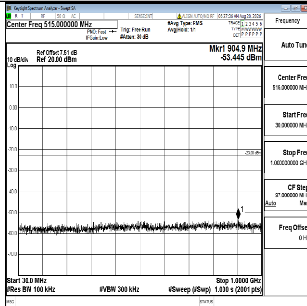
Band4-20MHz-16QAM-20175-1RB#0-30~1000-PASS
