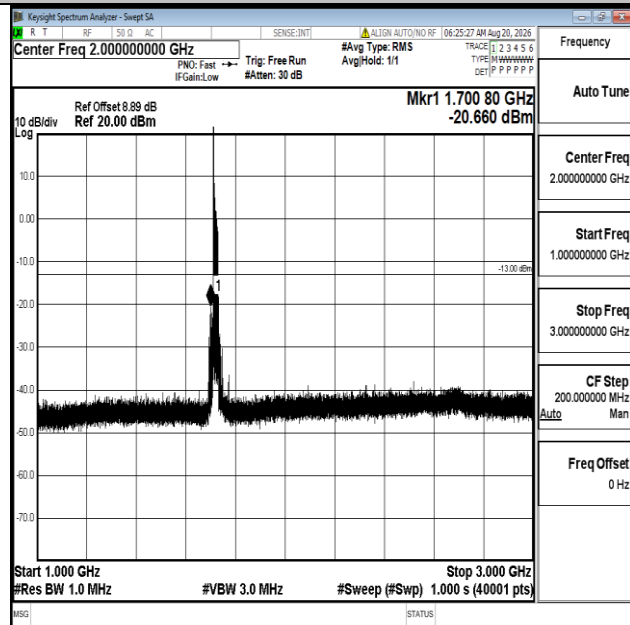
Band4-20MHz-QPSK-20050-1RB#0-1000~3000-PASS
