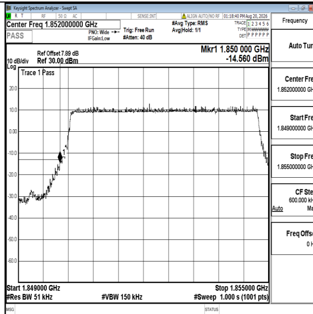
Band25-5MHz-QPSK-26065-25RB#0-PASS
