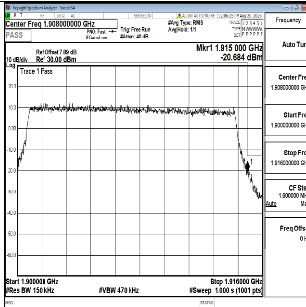
Band25-15MHz-16QAM-26615-75RB#0-PASS
