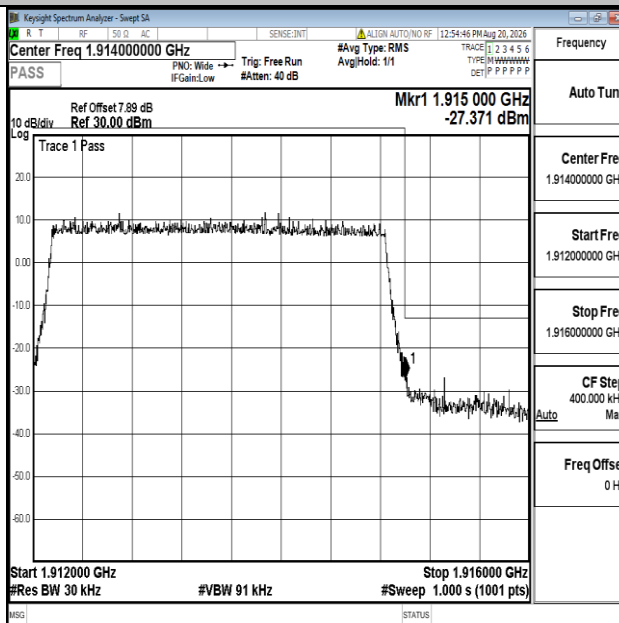
Band25-3MHz-16QAM-26675-15RB#0-PASS
