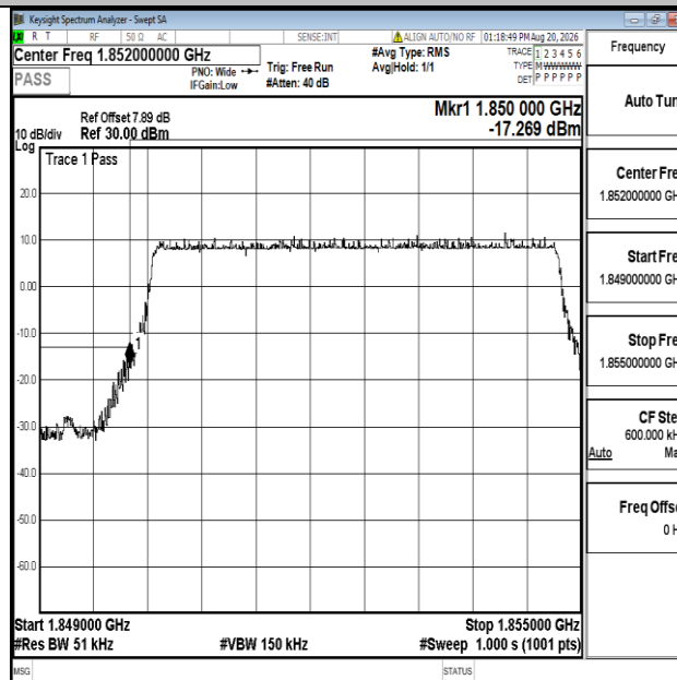
Band25-5MHz-16QAM-26065-25RB#0-PASS
