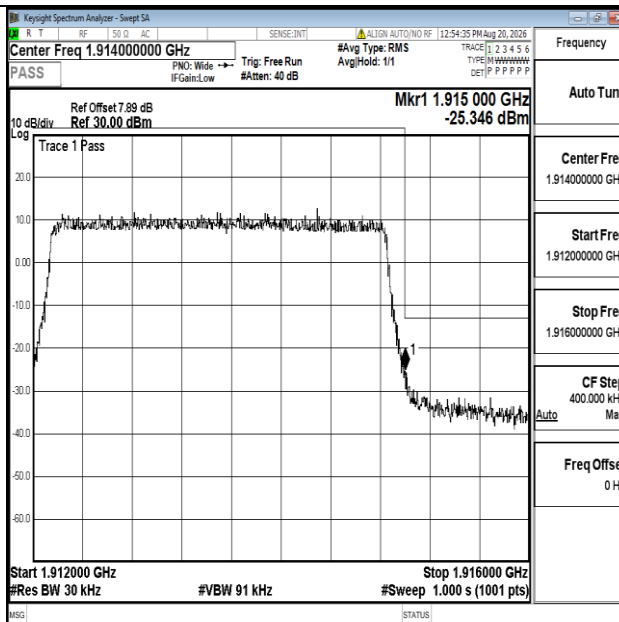
Band25-3MHz-QPSK-26675-15RB#0-PASS
