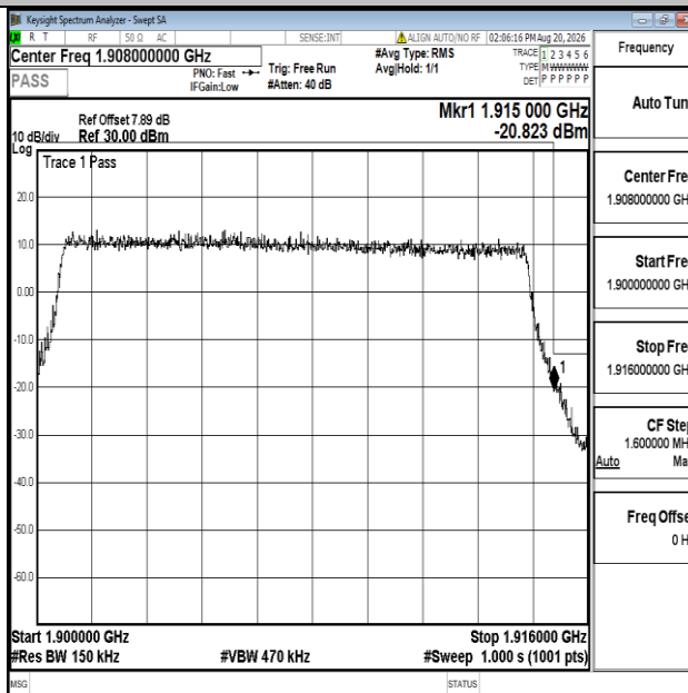
Band25-15MHz-QPSK-26615-75RB#0-PASS
