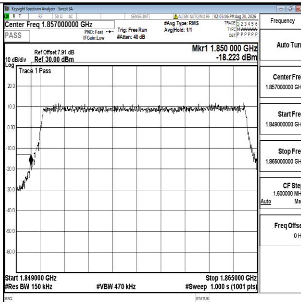
Band25-15MHz-16QAM-26115-75RB#0-PASS
