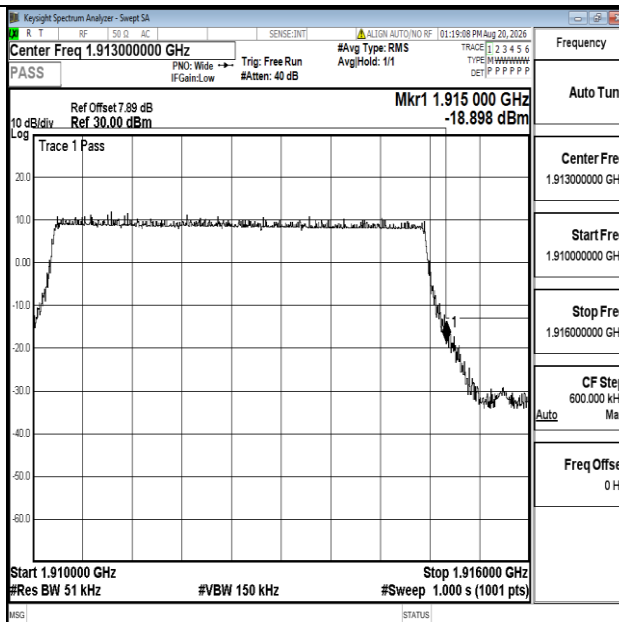
Band25-5MHz-16QAM-26665-25RB#0-PASS
