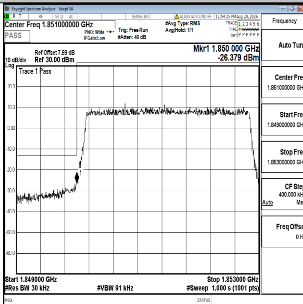
Band25-3MHz-16QAM-26055-15RB#0-PASS
