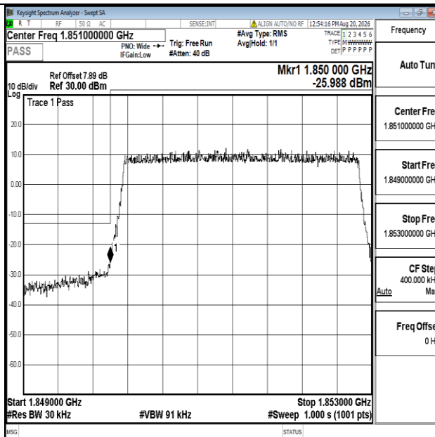
Band25-3MHz-QPSK-26055-15RB#0-PASS
