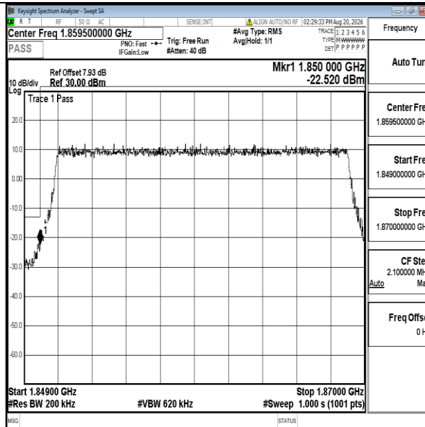
Band25-20MHz-16QAM-26140-100RB#0-PASS
