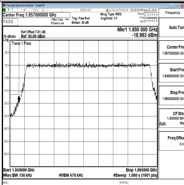
Band25-15MHz-QPSK-26115-75RB#0-PASS
