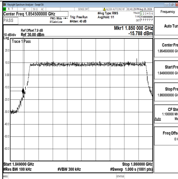
Band25-10MHz-16QAM-26090-50RB#0-PASS
