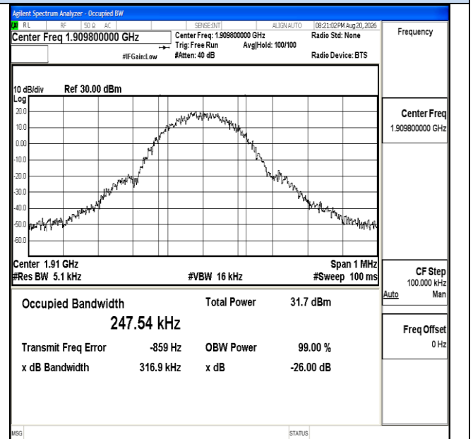
Channel 810 / 1909.8 MHz
