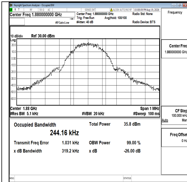
Channel 661 / 1880.0MHz
