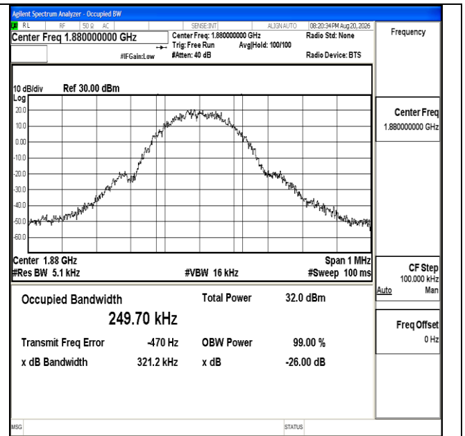
Channel 661 / 1880.0MHz
