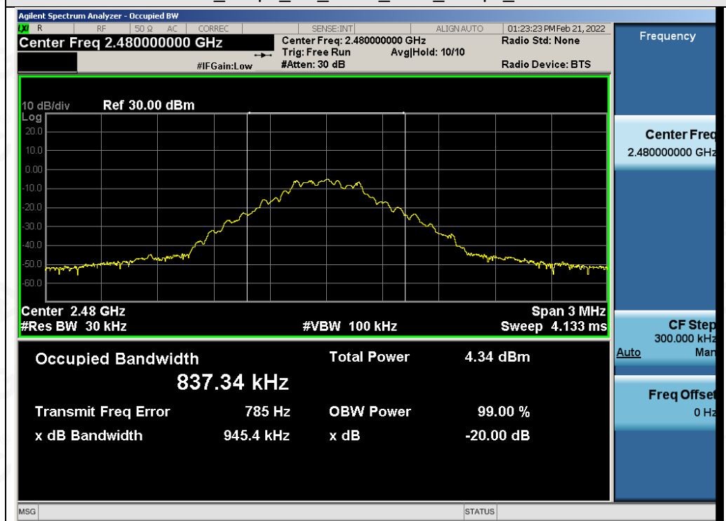
Test_Graph_BR_ANT1_2480_1Mbps_OBW
