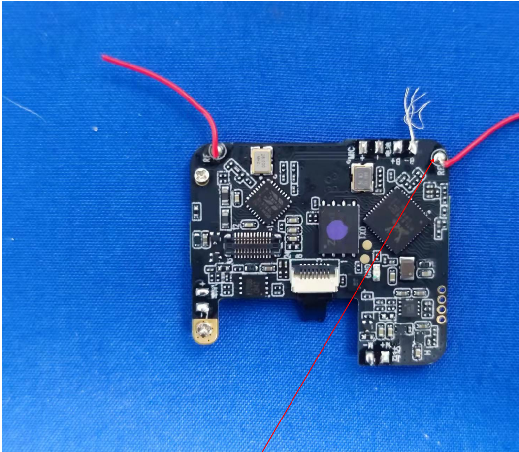
Integral antenna
