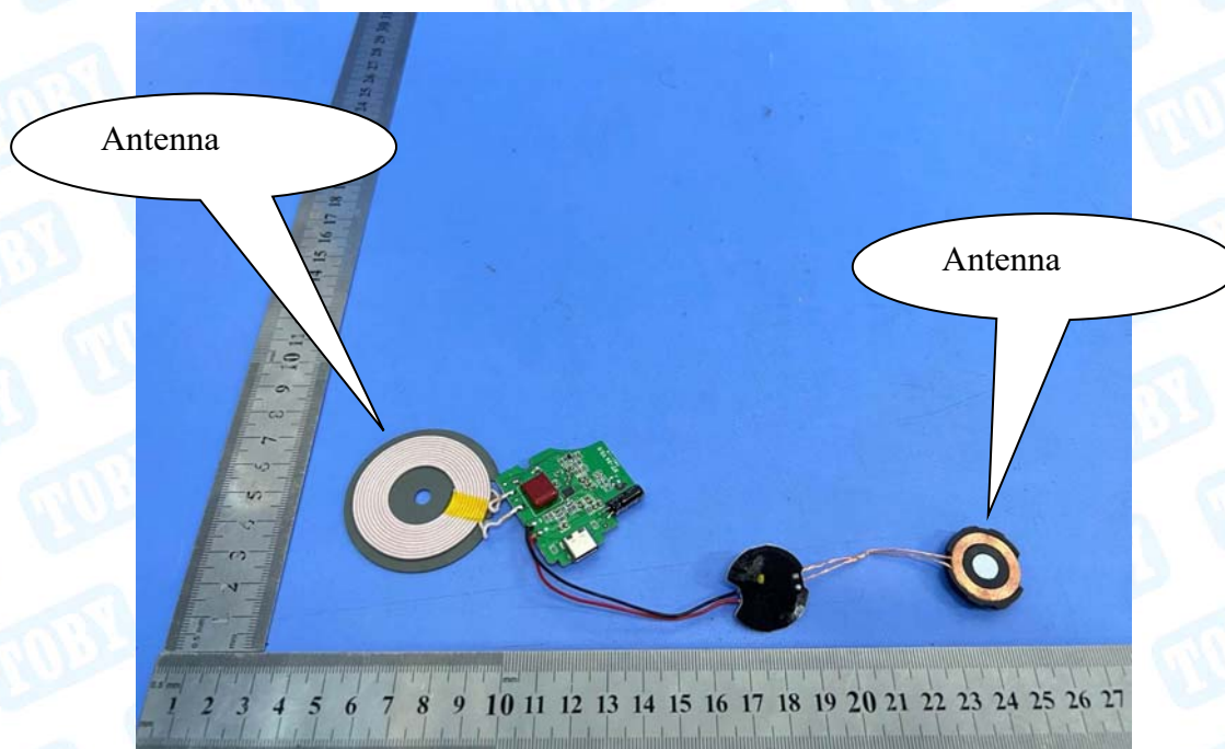
Photo 8 Appearance of PCB
