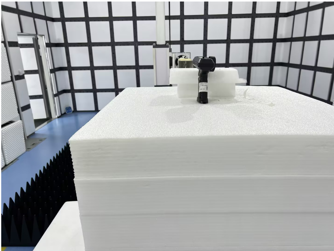
Radiated Emission - Front View (18GHz – 25GHz)
