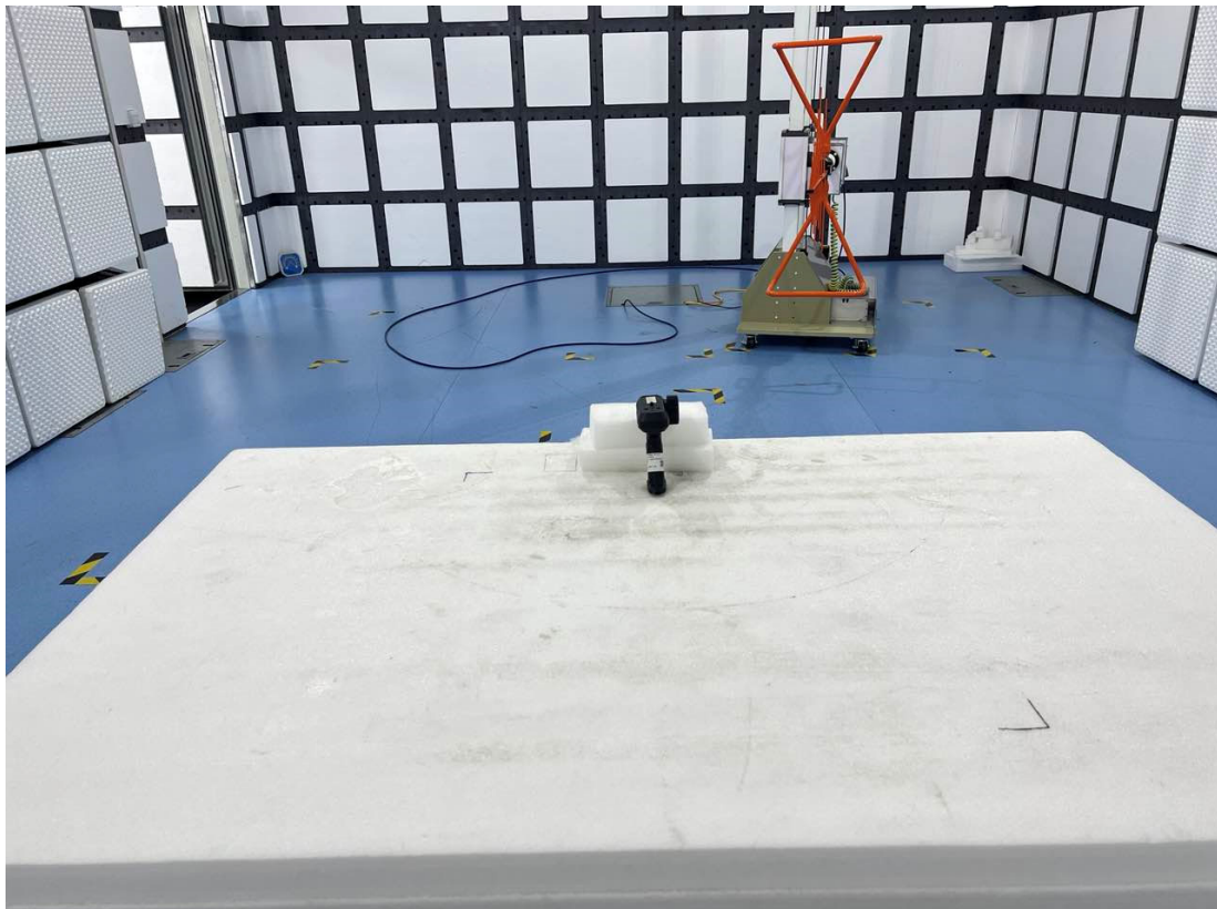
Radiated Emission - Front View (30MHz-1GHz)
