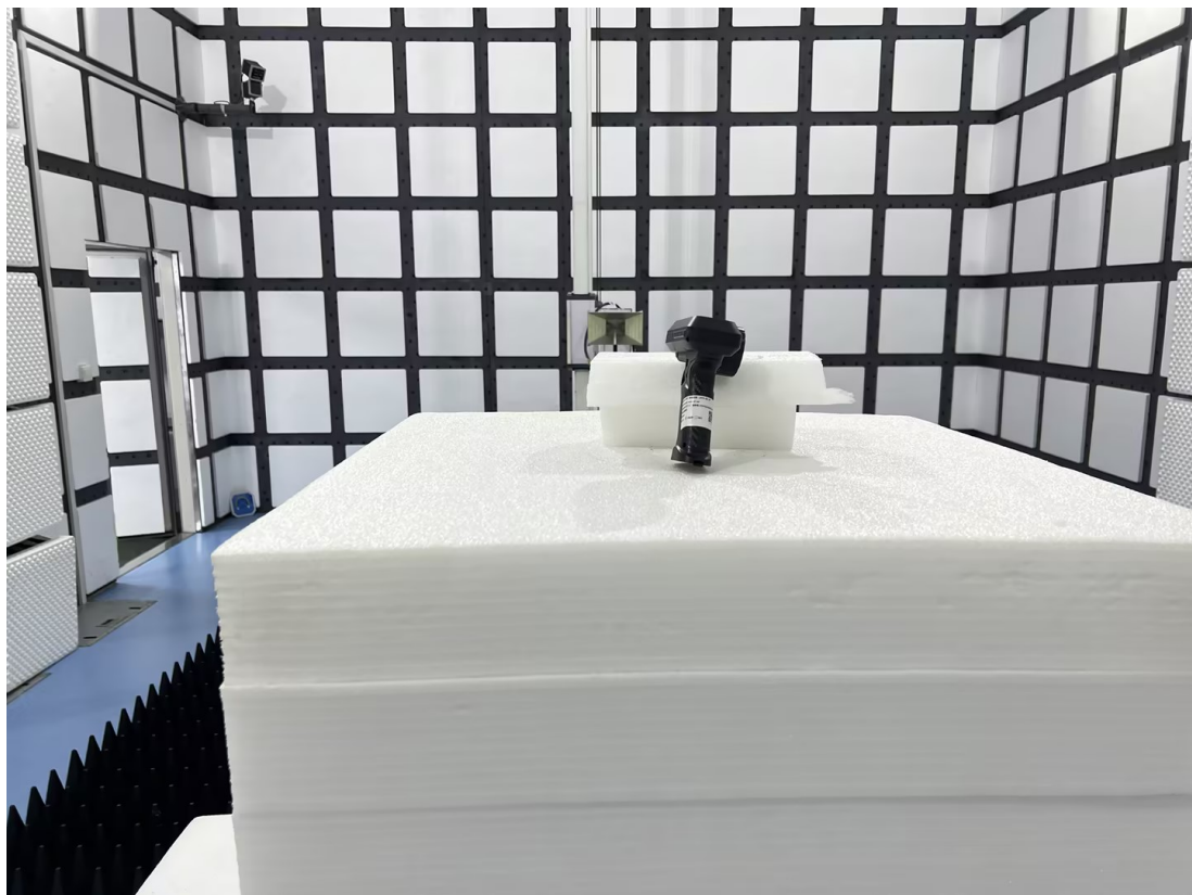
Radiated Emission - Front View (1GHz – 18GHz)
