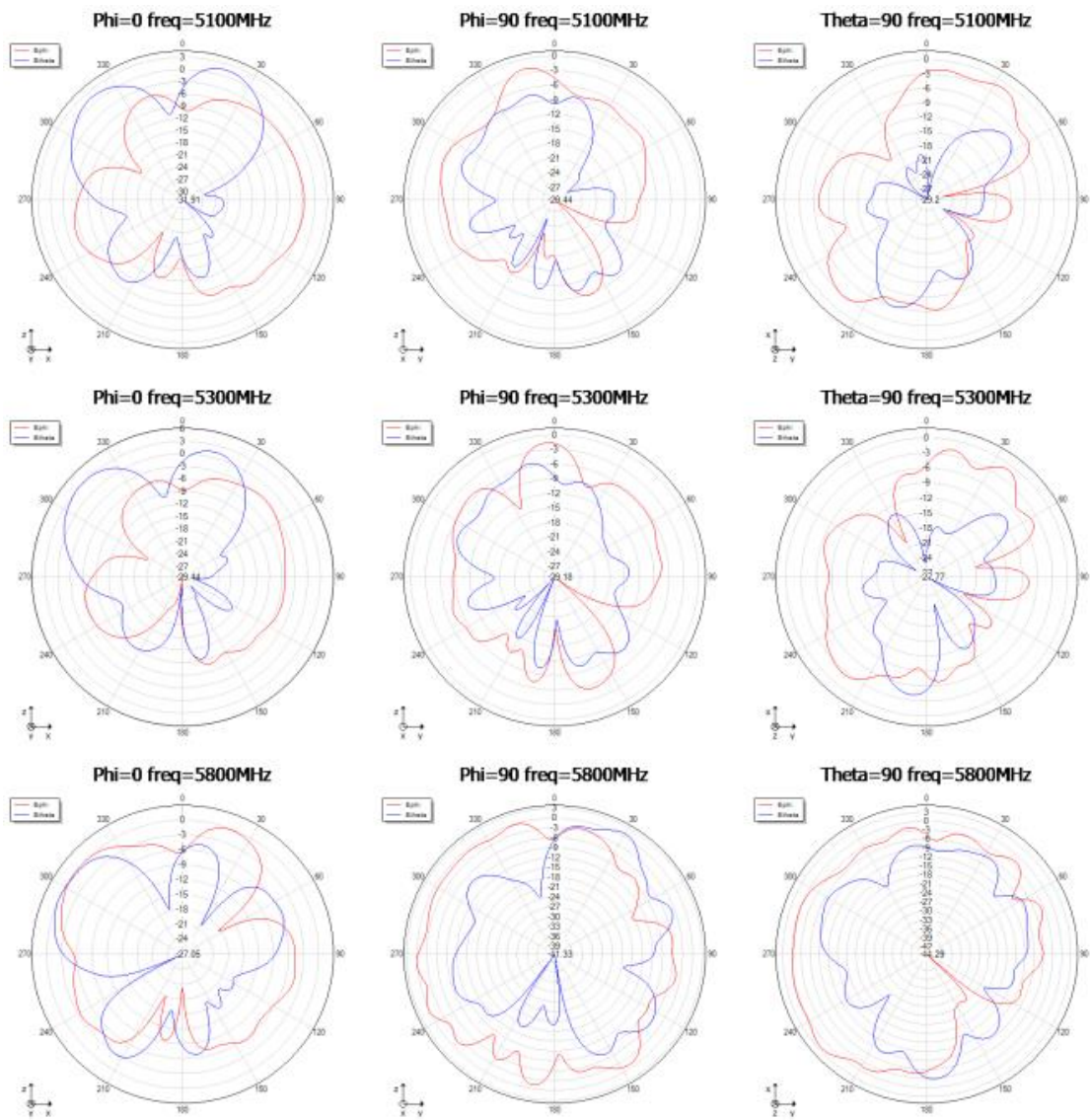
WiFi antenna 3D_Graphs(Total)
