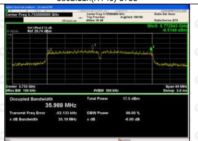
5802.11n(HT40)-5755
