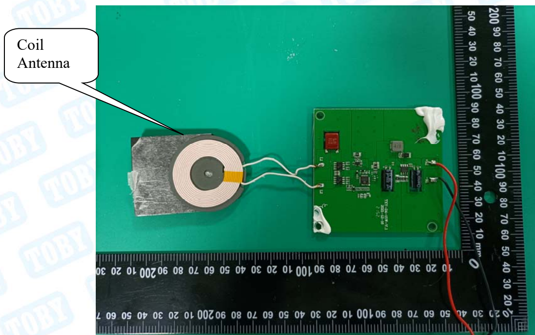
Photo 13 Appearance of PCB
