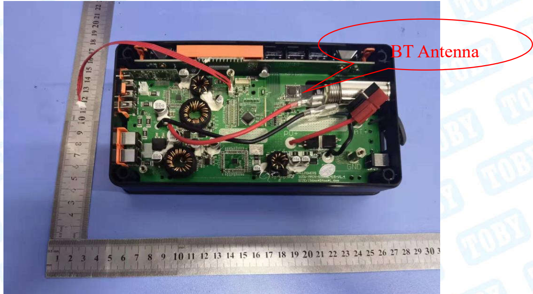
Photo 10 Appearance of PCB
