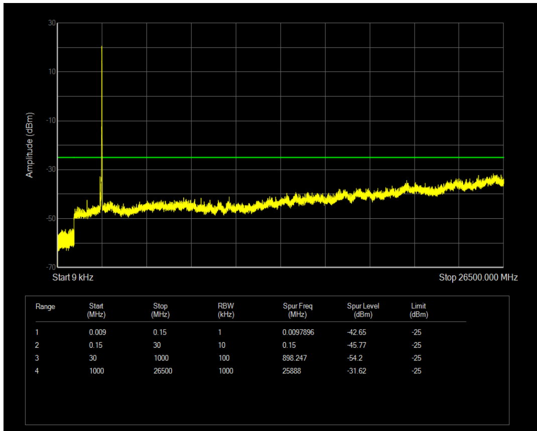
Band41 QAM16 BW=20MHz Channel=41240 RB Size=1 Position=#0
