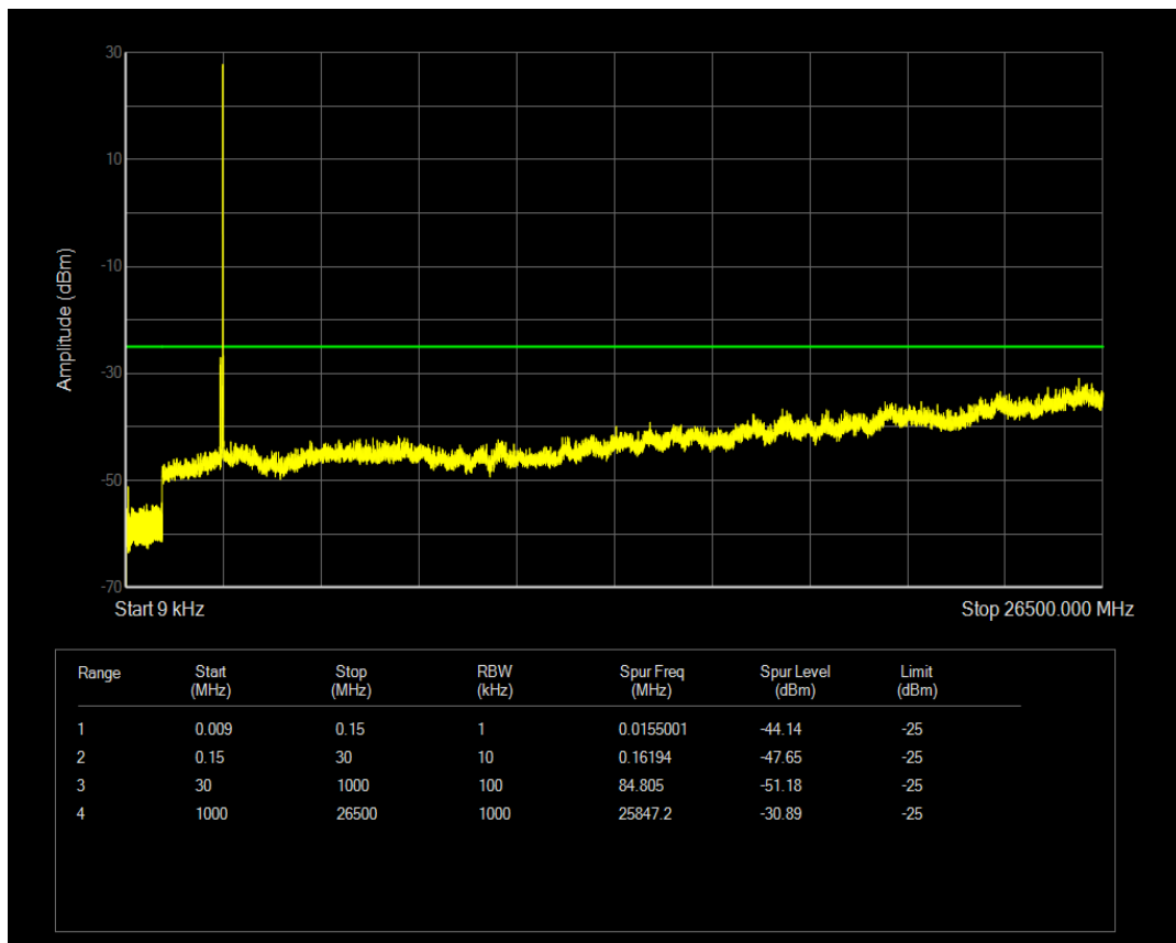
Band41 QAM16 BW=20MHz Channel=41240 RB Size=100 Position=#0
