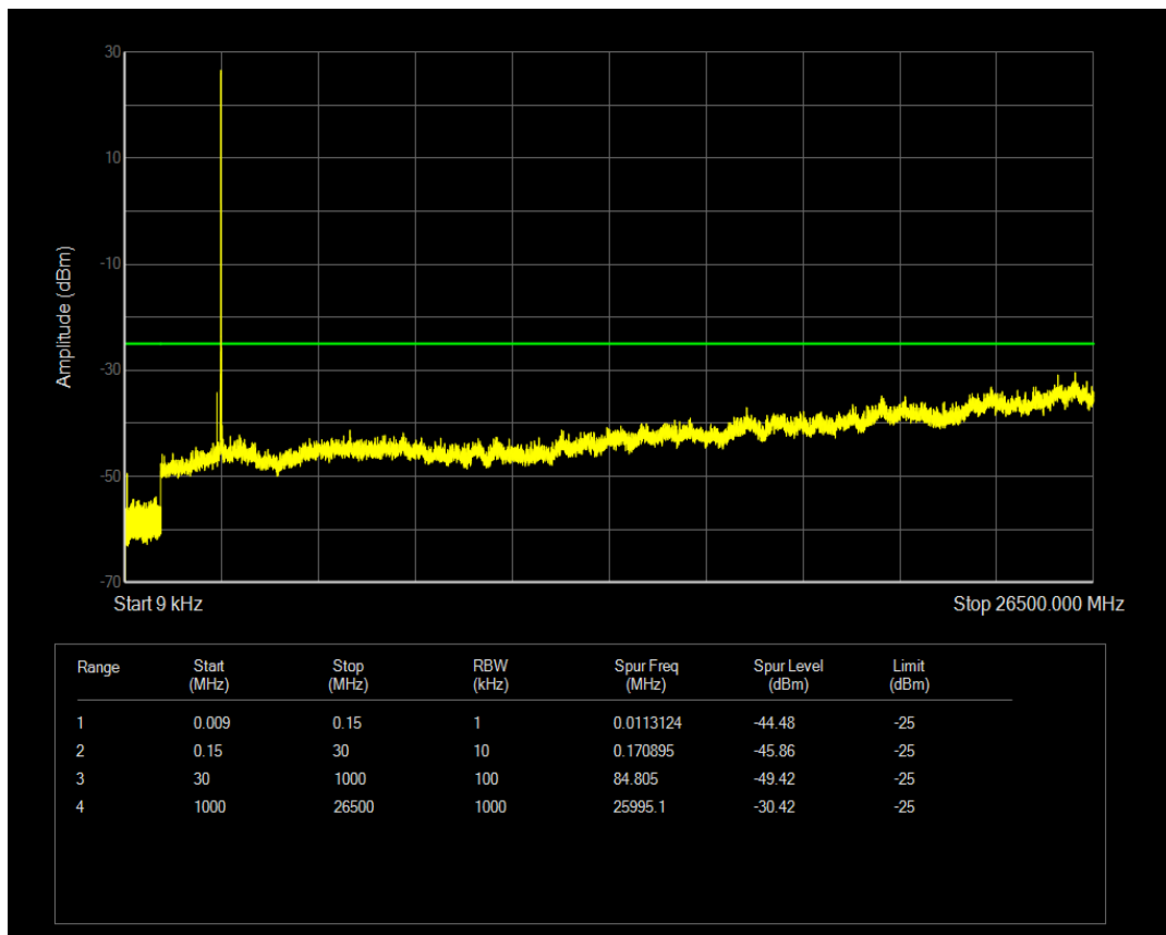
Band41 QPSK BW=20MHz Channel=41240 RB Size=100 Position=#0
