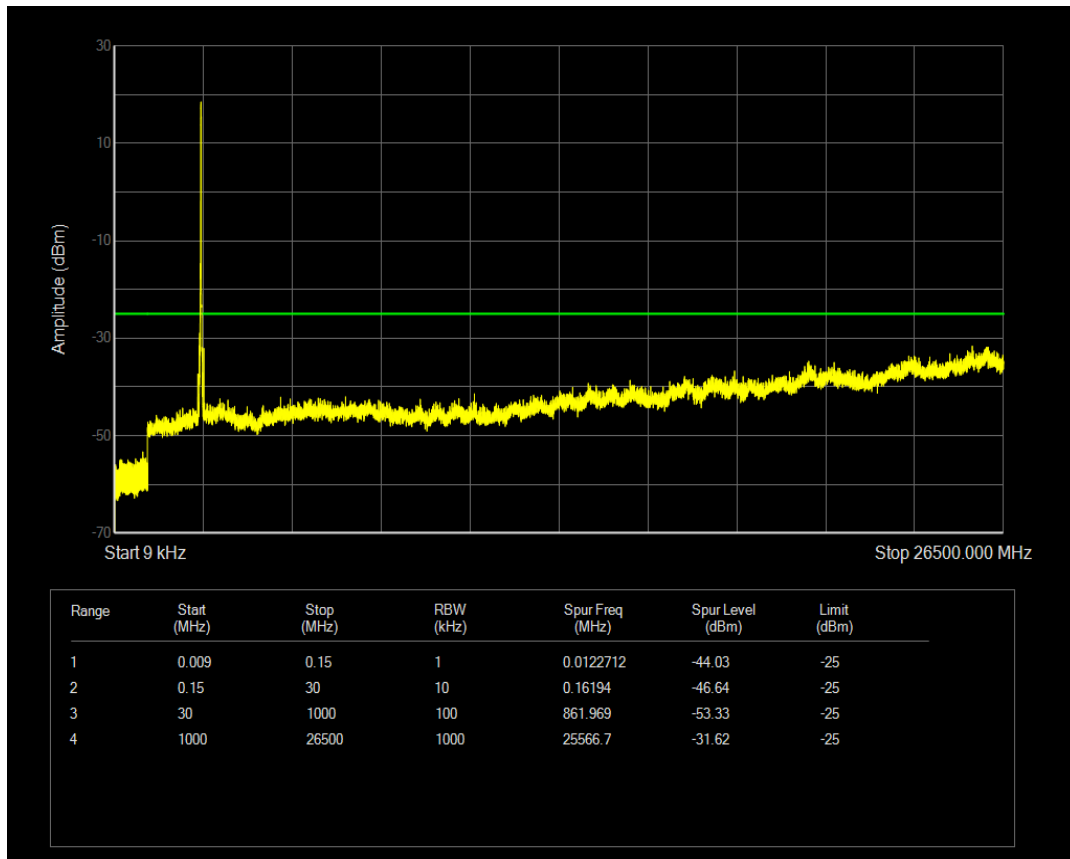
Band41 QPSK BW=20MHz Channel=41240 RB Size=1 Position=#0
