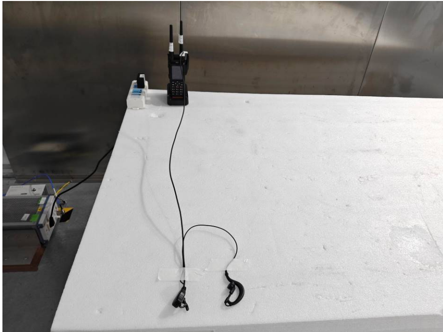
CE - Side View – Mode 1
