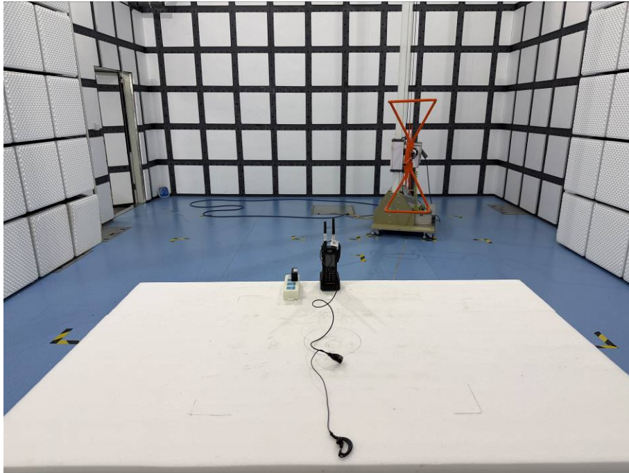
RSE - Back View (Below 1 GHz) – Mode 1
