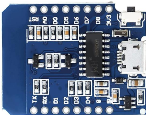
ESP8266-MINI BOTVIEW
