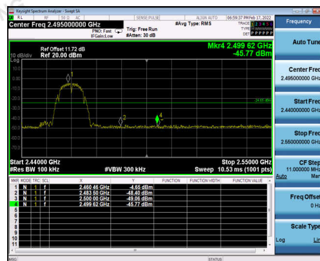
Right bandedge
