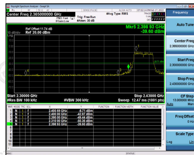
Left bandedge
