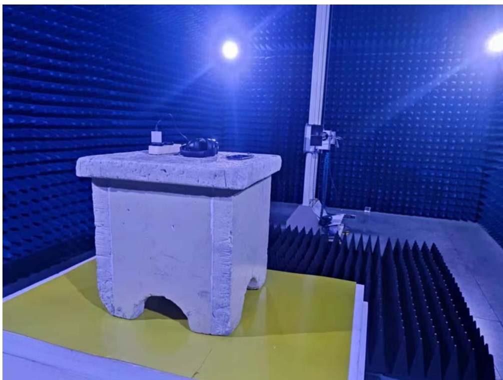
Photo of Radiated Emission Measurement Above 1GHz
