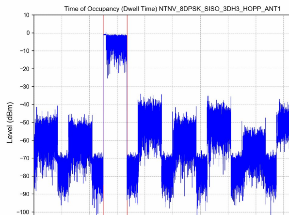
3DH3
