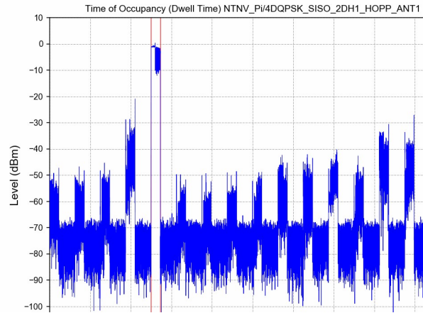
2DH1
