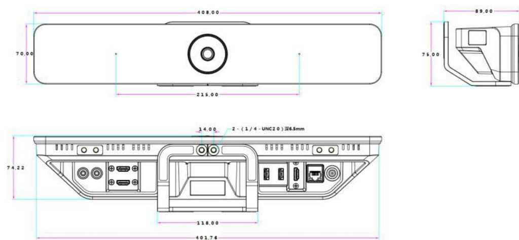
Figure 1.0 UT30 Dimension
