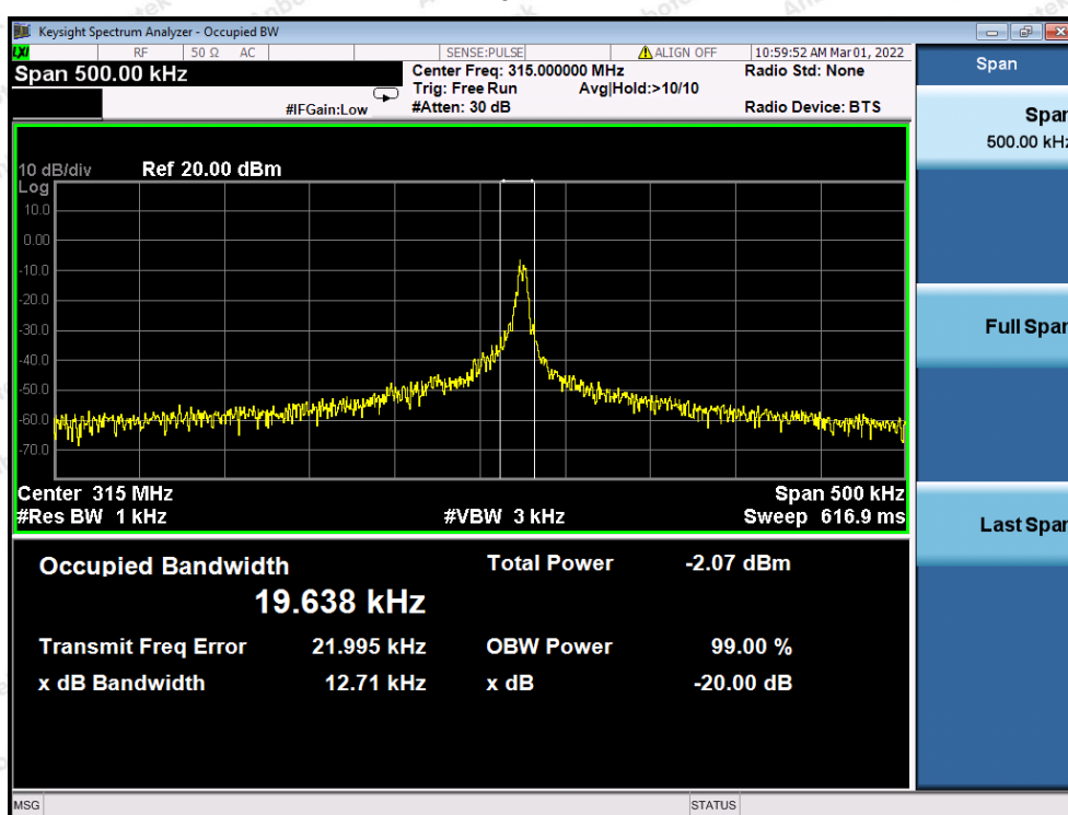
315 MHz Plot of 20DB Bandwidth
