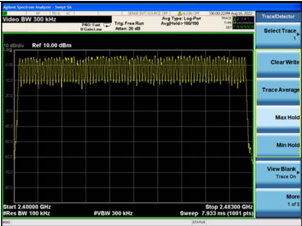
GFSK Modulation
