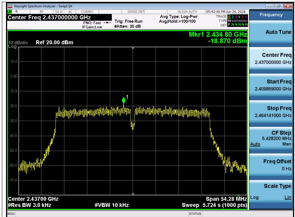
Test_Graph_802.11n40_Chain A_2437_MCS0_PSD
