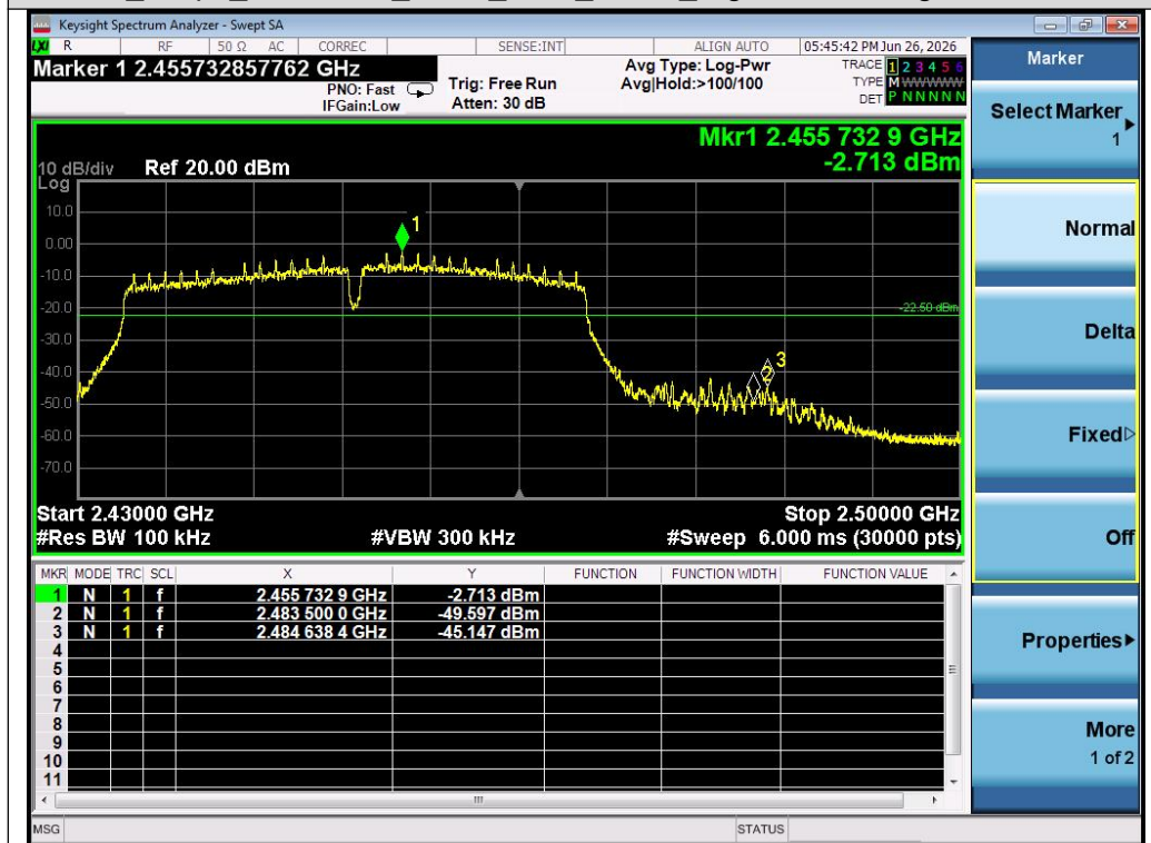
Test Graph 802.11n40 ANT1 2452 MCS0 Higher Band Edge Emissions
