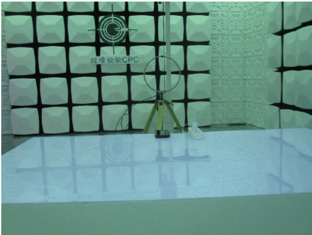
Setup Photo FCC ID: 2A4WMWZC-C01
