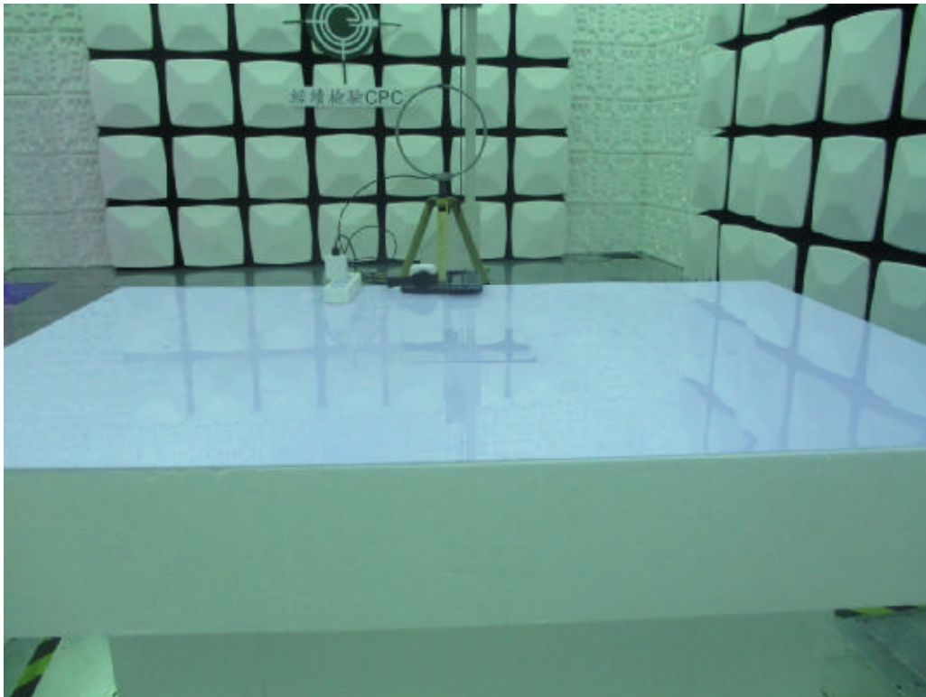
Setup Photo FCC ID: 2A4WMWZC-CW310
