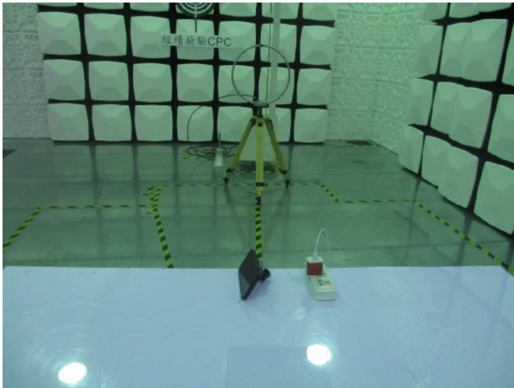
Setup Photo FCC ID: 2A4WMWZC-W107
