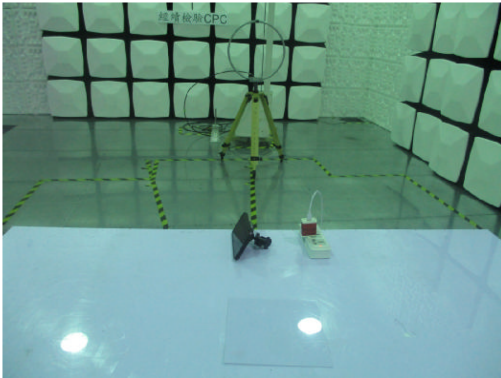
Setup Photo FCC ID: 2A4WMWZC-W112
