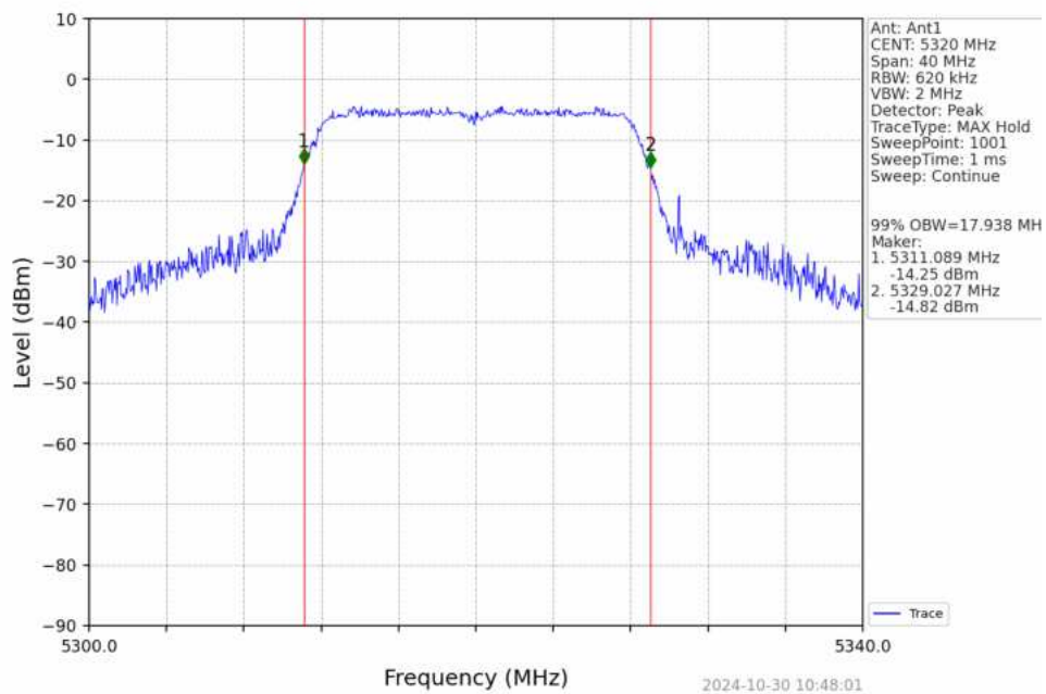
802.11a_HCH_5320MHz_Ant1_NTNV
