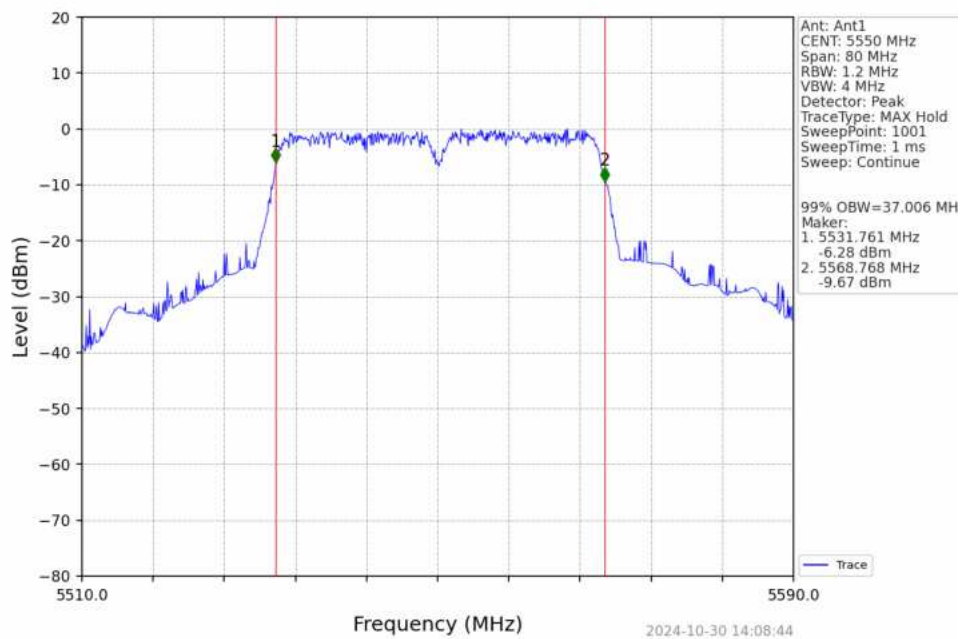
802.11n(HT40)_MCH_5550MHz_Ant1_NTNV
