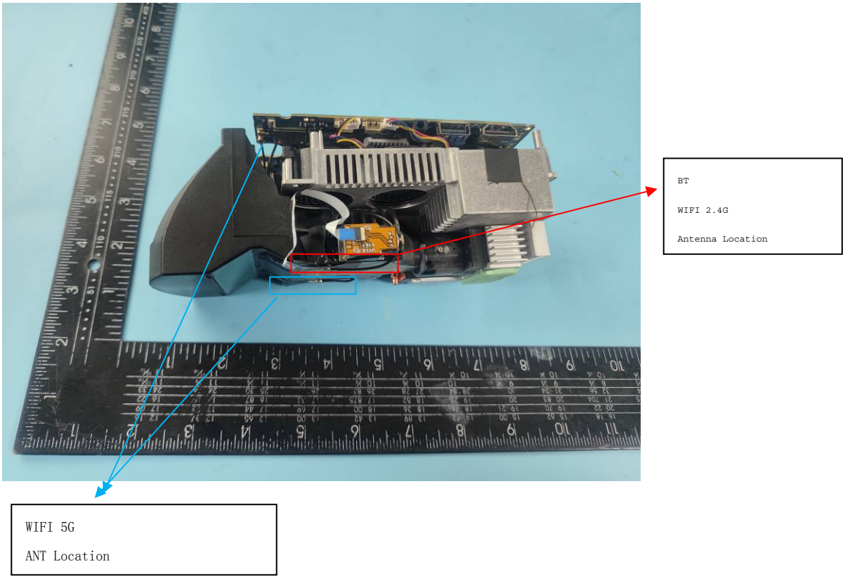
INTERNAL PHOTO OF SAMPLE PCB
