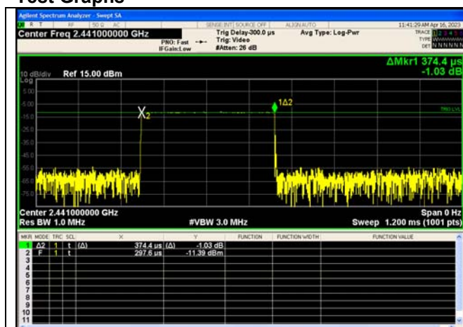
Pulse Width GFSK_DH1
