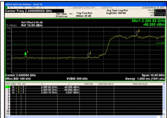
Out Of Band Emission(Left) 8DPSK_3-DH5_Channel Hopping
