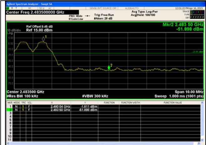
Out Of Band Emission(Right) GFSK_DH5_Channel Hopping
