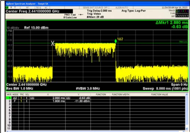
Pulse Width 8DPSK_3-DH5
