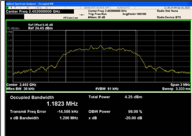
8DPSK 3-DH5 Channel 0
