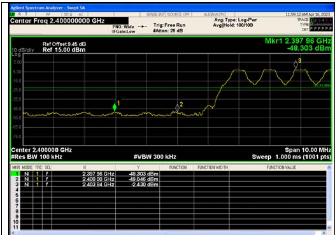
Out Of Band Emission(Left) GFSK_DH5_Channel Hopping
