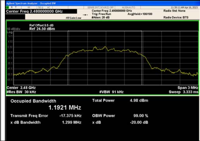
8DPSK 3-DH5 Channel 78
