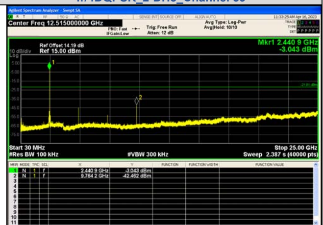
Spurious Emissions \pi/4 DQPSK_2-DH5_Channel 39
