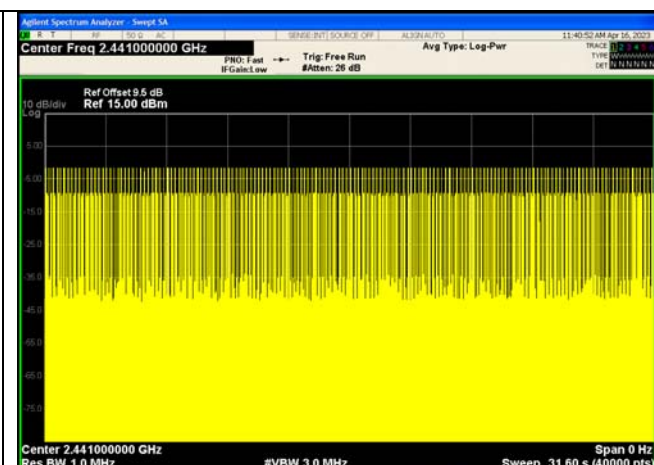
Number of Pulses in 31.6 seconds GFSK_DH1
