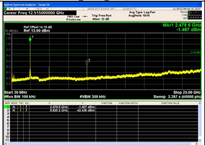
Spurious Emission 8DPSK_3-DH5_Channel 78
