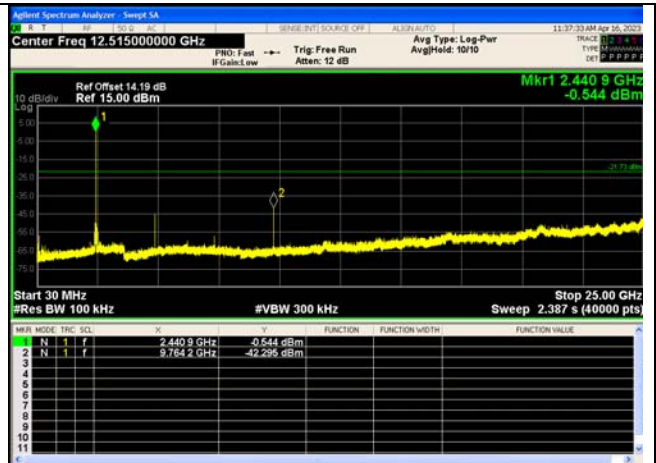
Spurious Emissions 8DPSK_3-DH5_Channel 39
