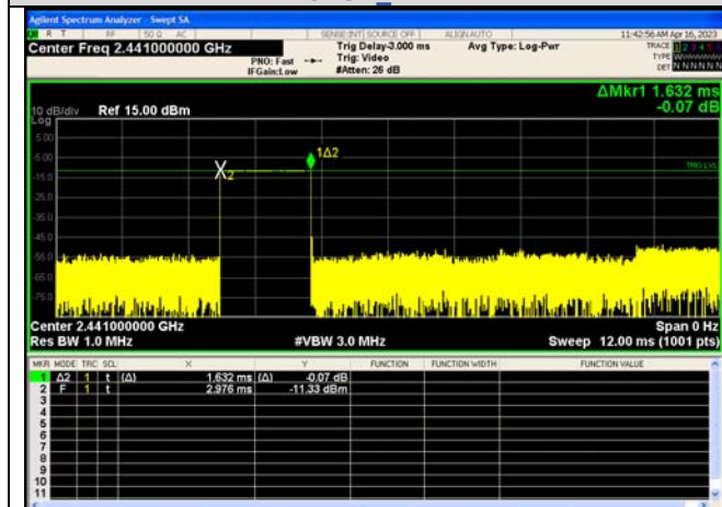
Pulse Width GFSK_DH3
