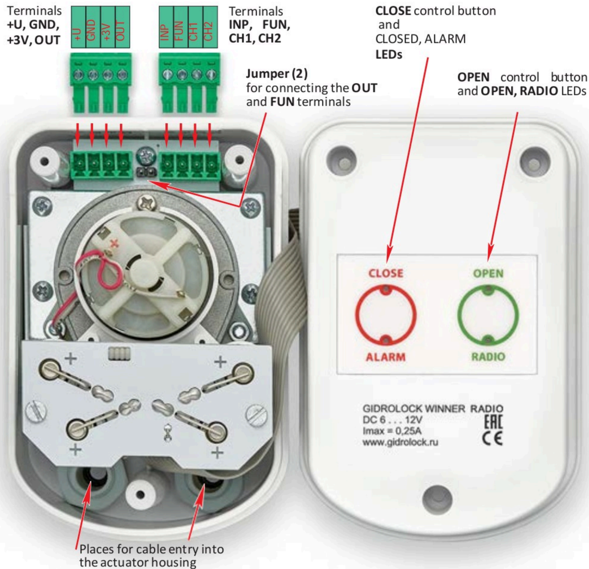
Photo 6. Electric actuator for ball valve control, with cover removed
