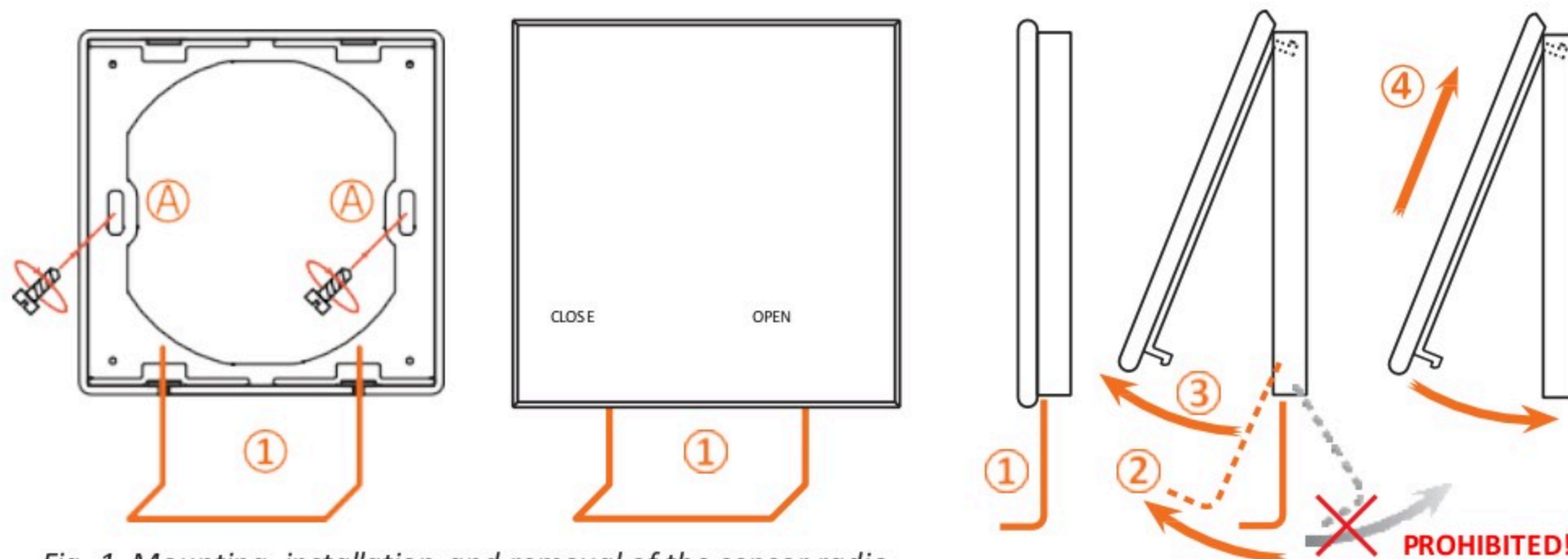
Fig. 1. Mounting, installation and removal of the sensor radio remote control
