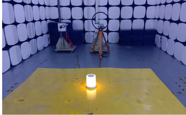
Radiated emission 30MHz~1GHz
