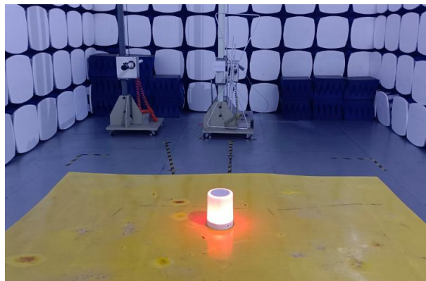
Radiated emission above 1GHz
