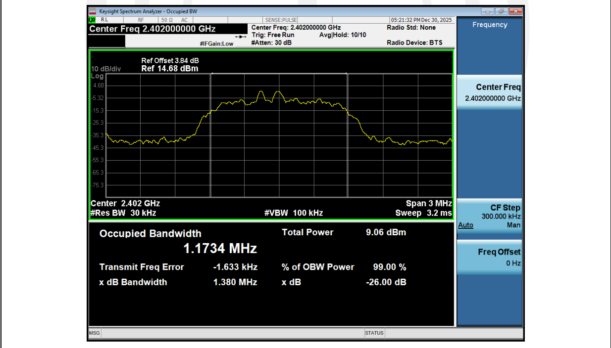
99%_Occupied_Bandwidth_NVNT_ANT1_2-DH1_2402_00
