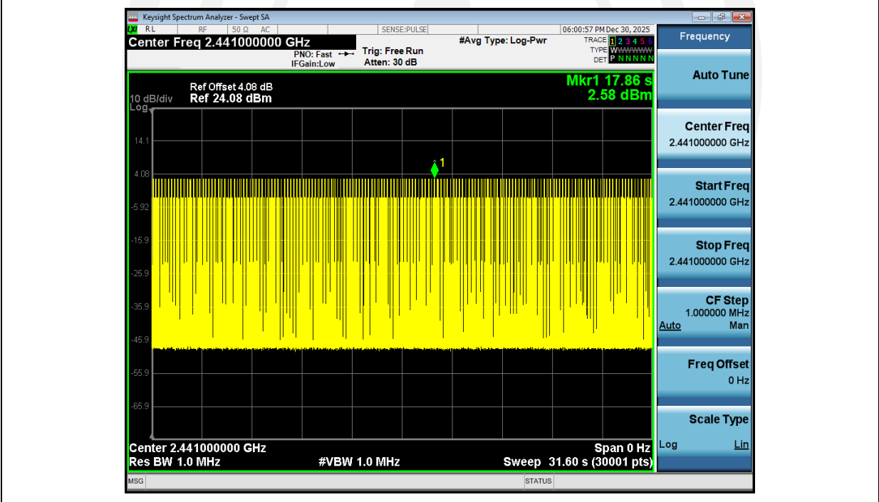
Dwell_Time (Hopping)_NVNT_ANT1_3-DH1_2441_00_Accumulated
