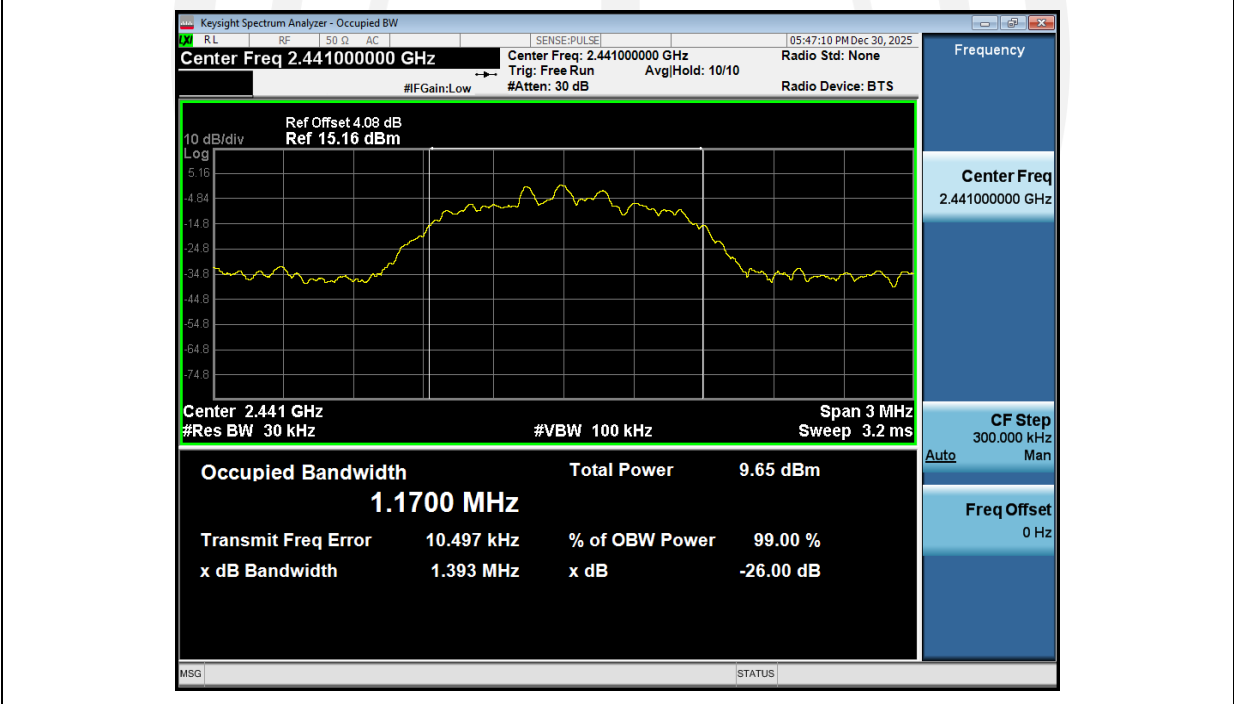
99%_Occupied_Bandwidth_NVNT_ANT1_3-DH1_2441_00
