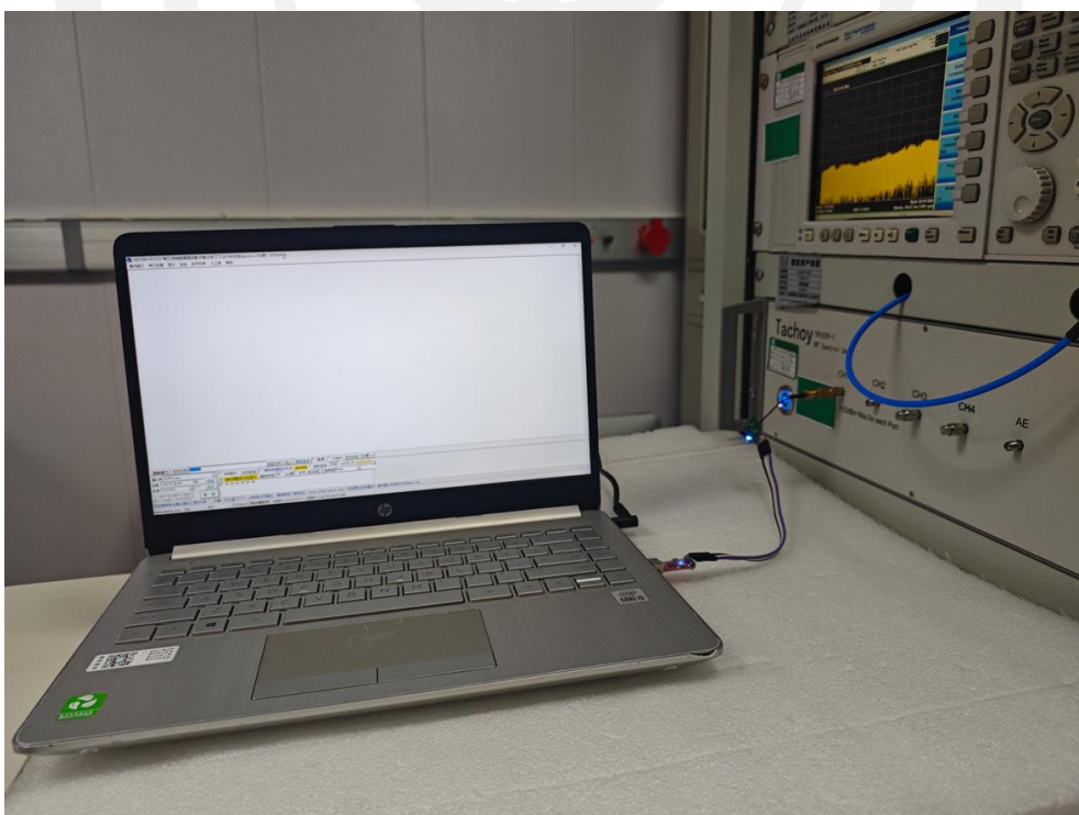
RF conducted Test (Right)
