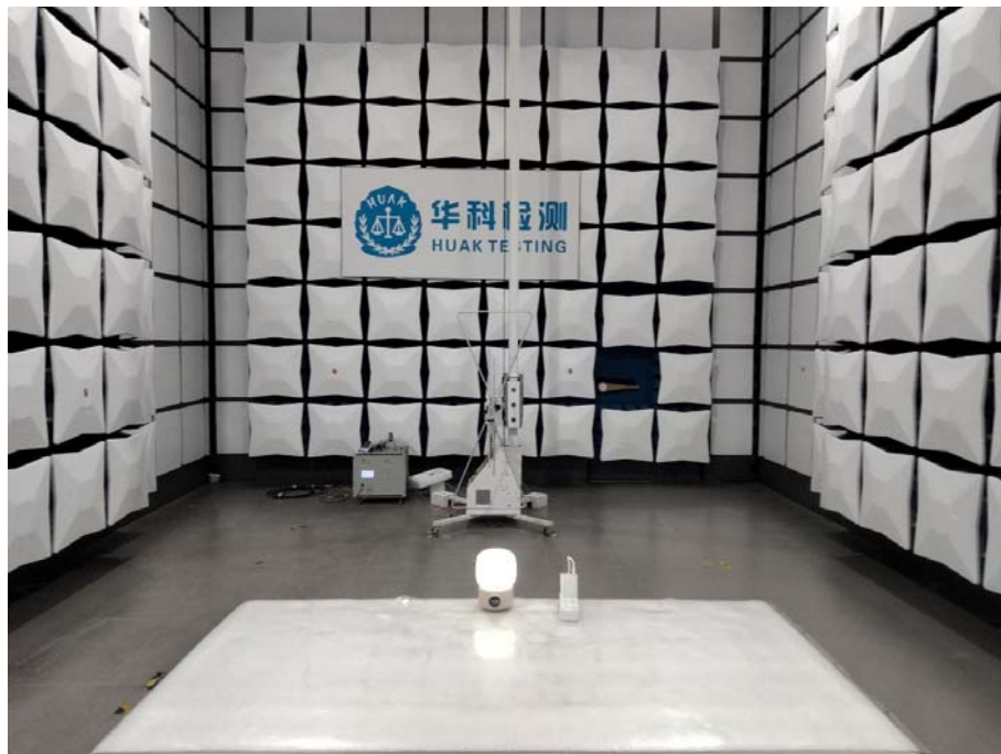
Model: S8 Radiated Emissions
