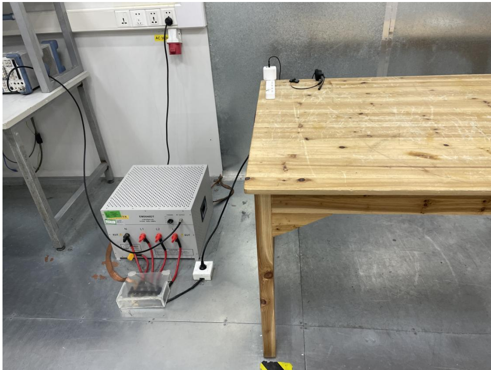
FCC ID: 2A4ZW-BH520 Photo of Conducted Emission Measurement
