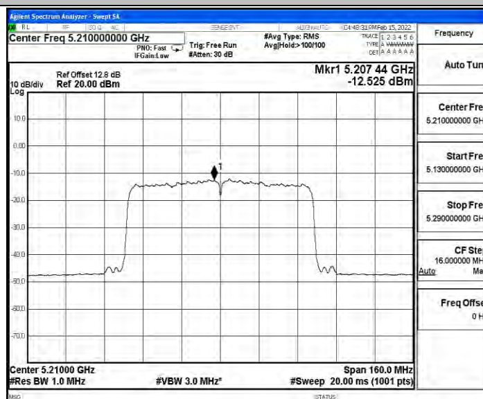
11AC80SISO_Ant4_5210
