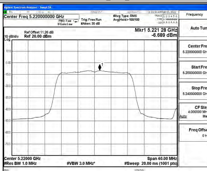
11N20SISO_Ant7_5220
