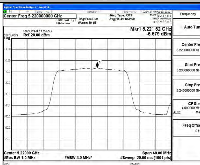
11N20SISO_Ant4_5220
