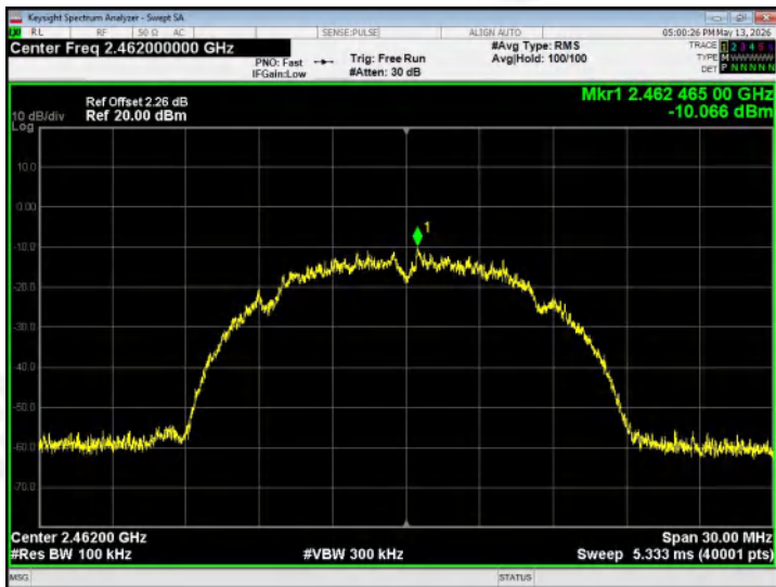
802.11b - Highest channel
