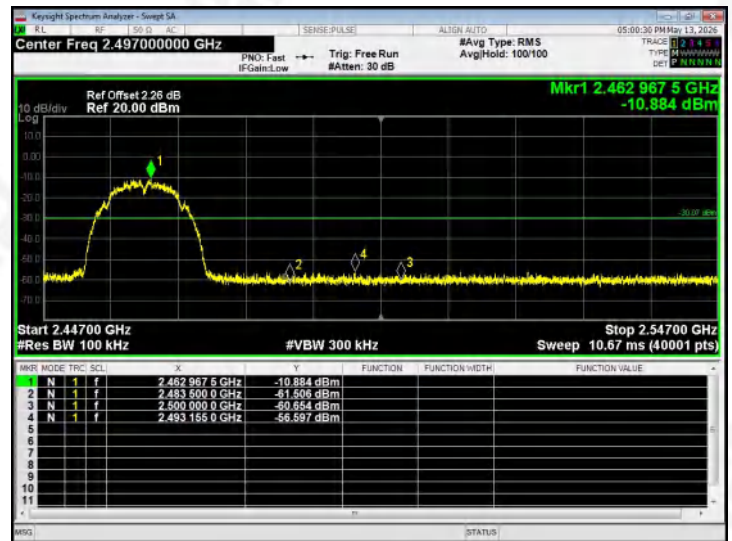
802.11b - Highest channel
