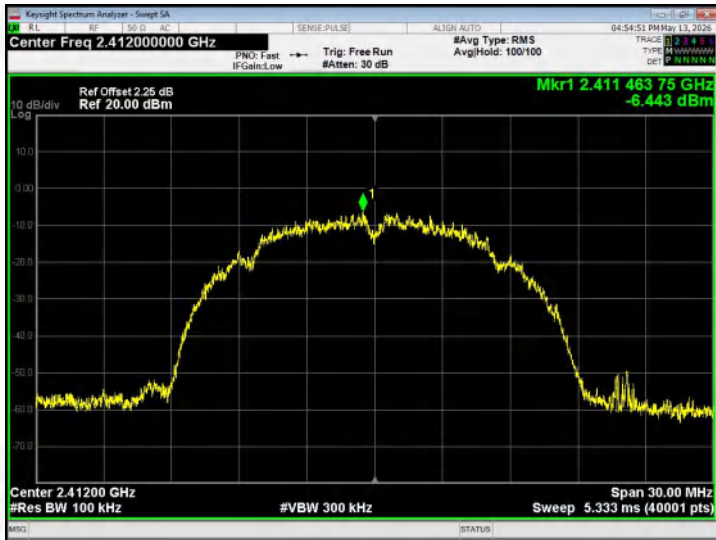
802.11b - Lowest channel
