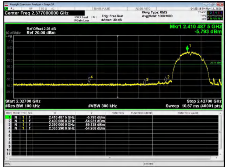
802.11b - Lowest channel
