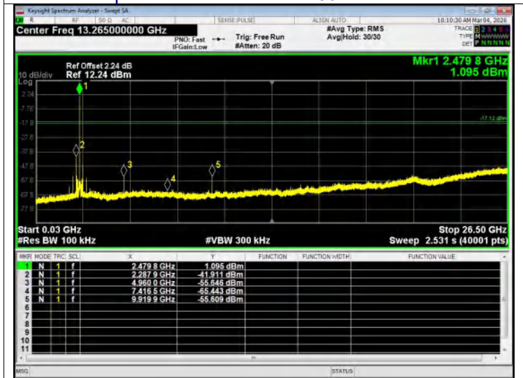
Tx. Spurious NVNT 1-DH1 2480MHz Emission
