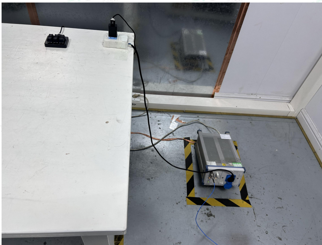
Fig. 3 RF Conducted
