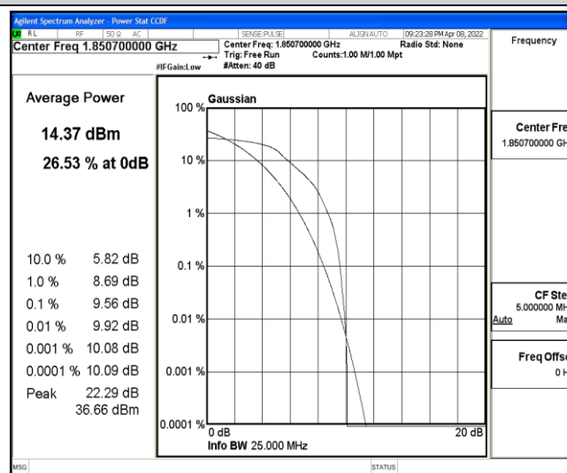
Band2-1.4MHz-16QAM-18607-6-0-Low-9.56-&lt;=13-PASS
