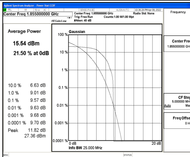
Band2-10MHz-QPSK-18650-1-0-Low-9.57-13-PASS
