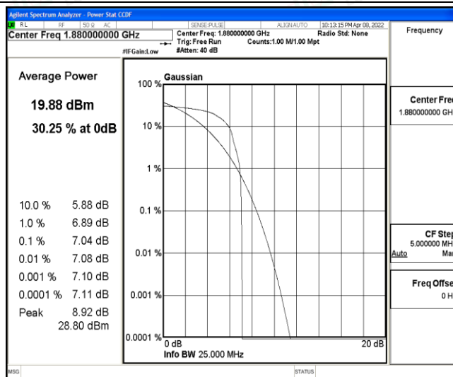
Band2-5MHz-16QAM-18900-1-0-Low-7.04-&lt;=13-PASS
