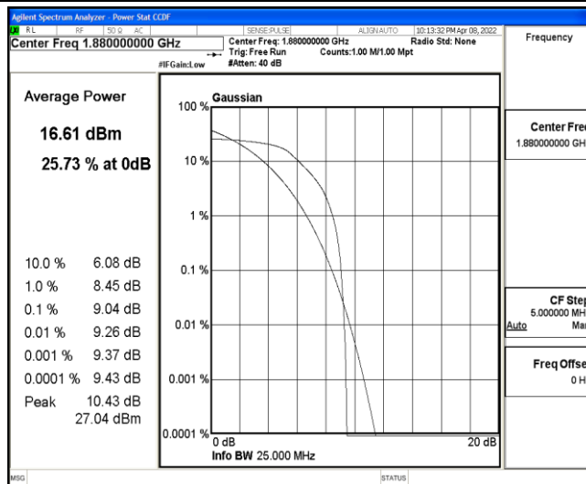
Band2-5MHz-16QAM-18900-6-0-Low-9.04-&lt;=13-PASS
