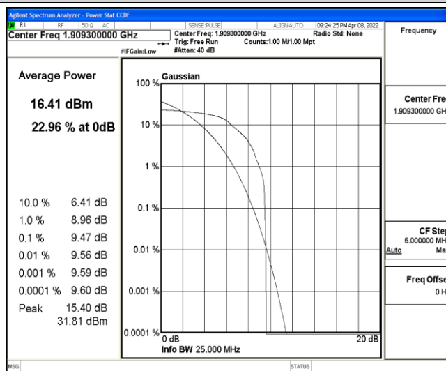
Band2-1.4MHz-QPSK-19193-1-0-High-9.47-&lt;=13-PASS
