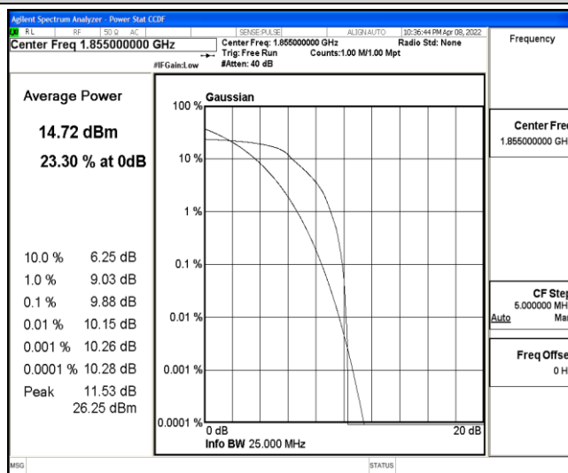
Band2-10MHz-QPSK-18650-6-0-Low-9.88-13-PASS
