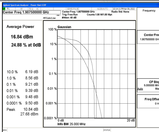
Band2-5MHz-16QAM-19175-6-0-High-9.21-13-PASS
