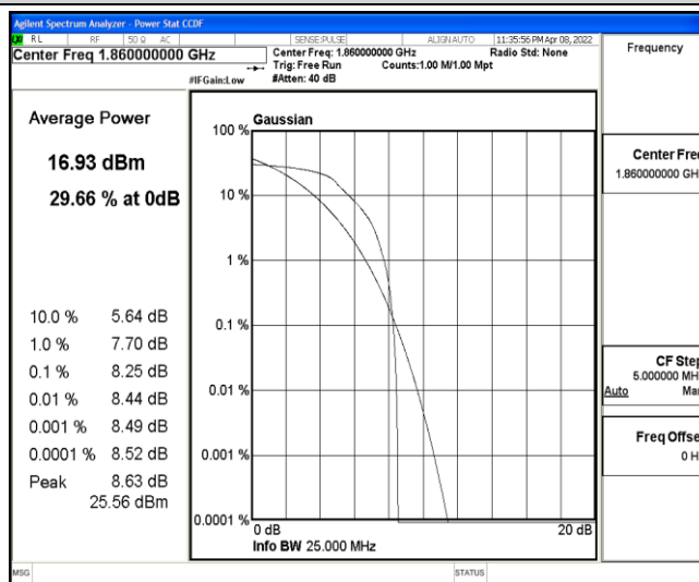
Band2-20MHz-QPSK-18700-6-0-Low-8.25-&lt;=13-PASS
