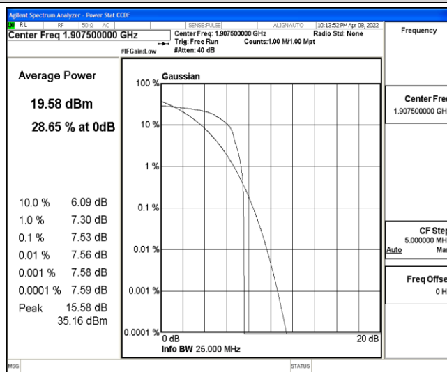
Band2-5MHz-16QAM-19175-1-0-High-7.53-&lt;=13-PASS
