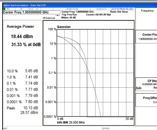
Band2-10MHz-16QAM-19150-1-0-High-7.74-&lt;=13-PASS
