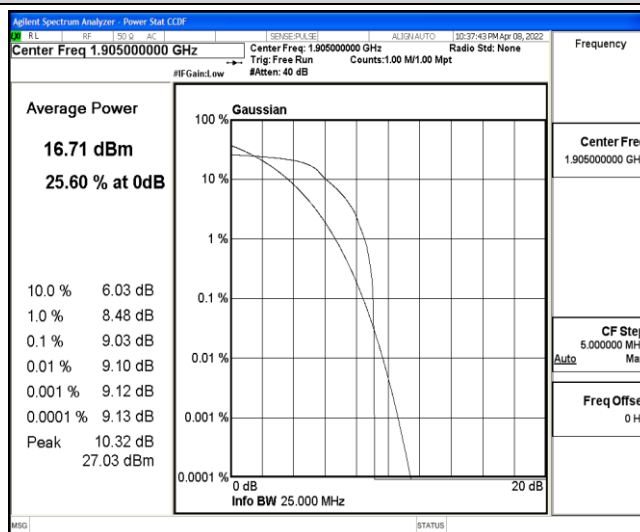
Band2-10MHz-QPSK-19150-1-0-High-9.03-&lt;=13-PASS
