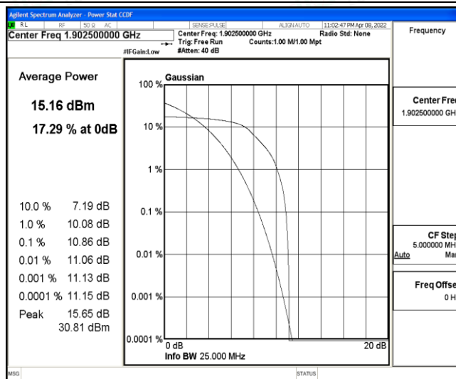
Band2-15MHz-16QAM-19125-6-0-High-10.86-&lt;=13-PASS
