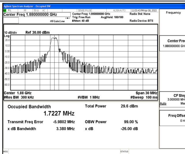
Band2-15MHz-QPSK-18900-6-0-Low-1.7227-3.380-PASS
