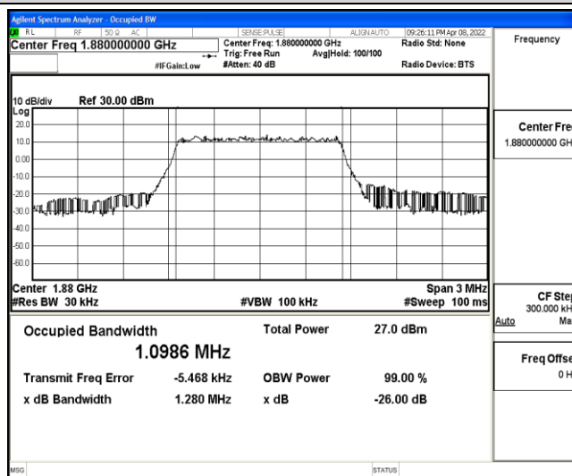
Band2-1.4MHz-16QAM-18900-6-0-Low-1.0986-1.280-PASS
