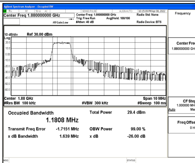
Band2-5MHz-QPSK-18900-6-0-Low-1.1808-1.639-PASS
