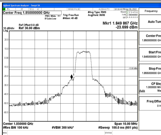
Band2-5MHz-16QAM-18625-6-0-Low--23.70-PASS
