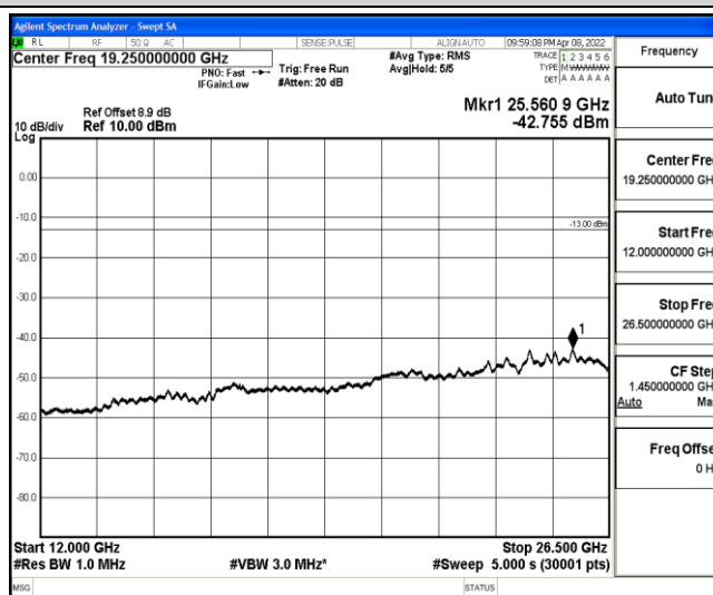
Band2-3MHz-QPSK-18900-1-0-Low-12000-26500--42.76-PASS
