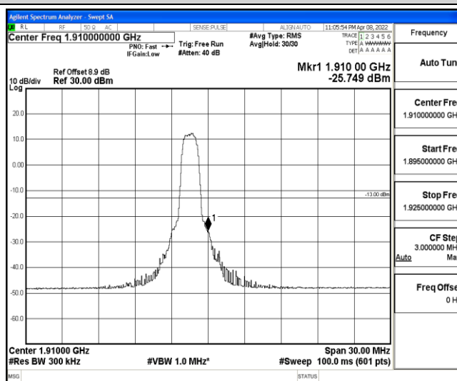
Band2-15MHz-16QAM-19125-6-0-High--25.75-PASS
