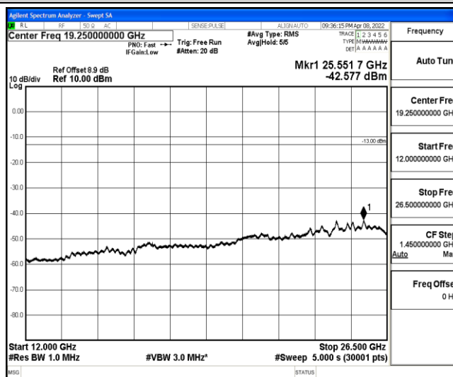
Band2-1.4MHz-16QAM-18900-1-0-Low-12000-26500--42.58-PASS
