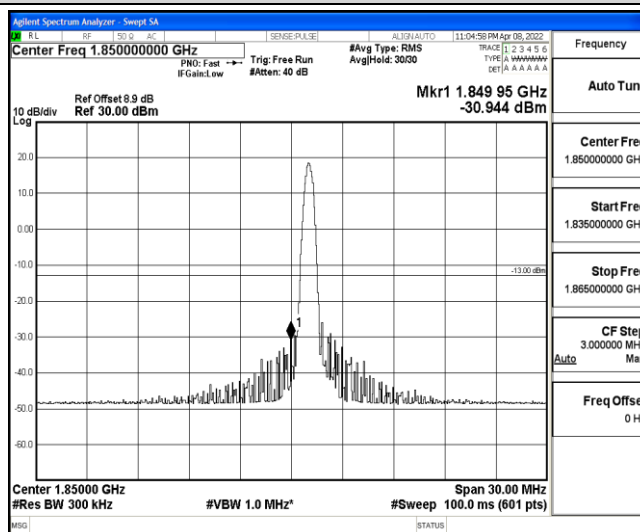
Band2-15MHz-16QAM-18675-1-0-Low--30.94-PASS
