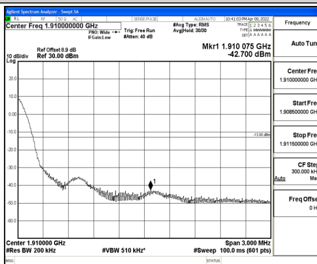
Band2-10MHz-16QAM-19150-1-0-High--42.70-PASS
