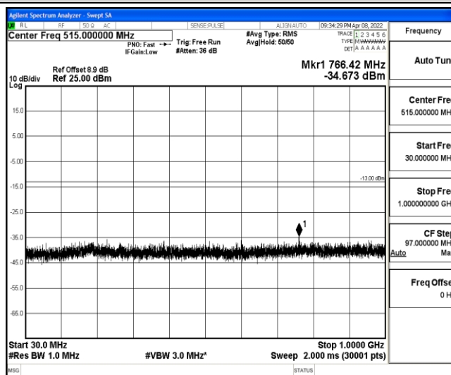
Band2-1.4MHz-16QAM-18900-1-0-Low-30-1000--34.67-PASS
