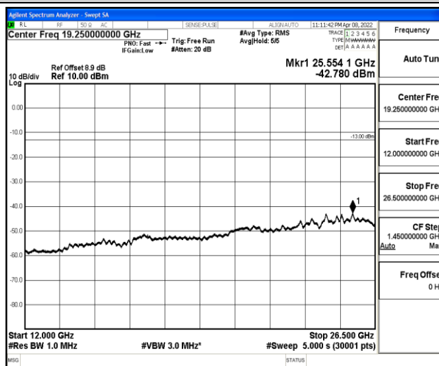
Band2-15MHz-QPSK-18900-1-0-Low-12000-26500--42.78-PASS
