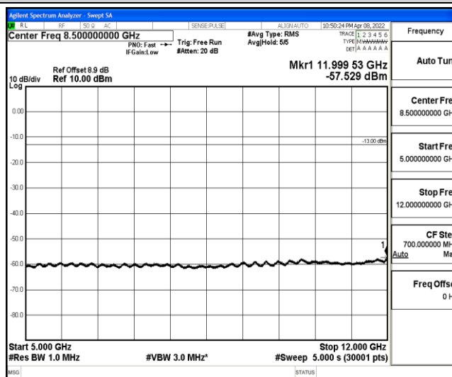
Band2-10MHz-QPSK-19150-1-0-High-5000-12000--57.53-PASS
