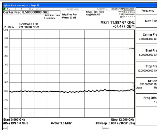
Band2-15MHz-QPSK-19125-1-0-High-5000-12000--57.48-PASS
