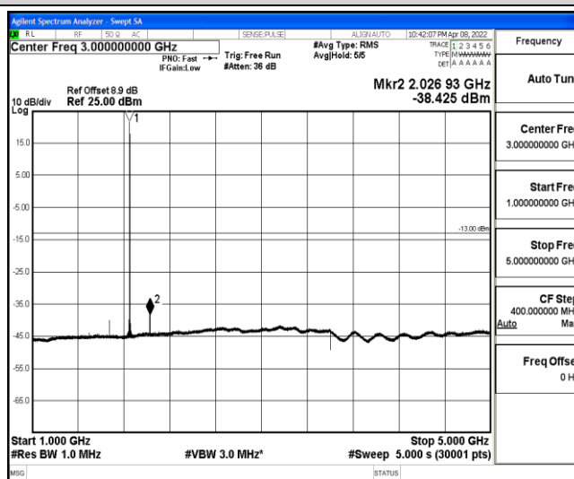
Band2-10MHz-QPSK-18650-1-0-Low-1000-5000--38.43-PASS
