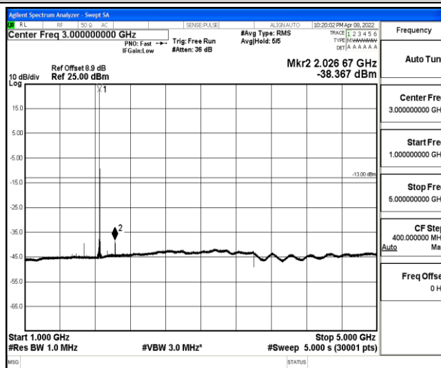
Band2-5MHz-16QAM-18625-1-0-Low-1000-5000--38.37-PASS
