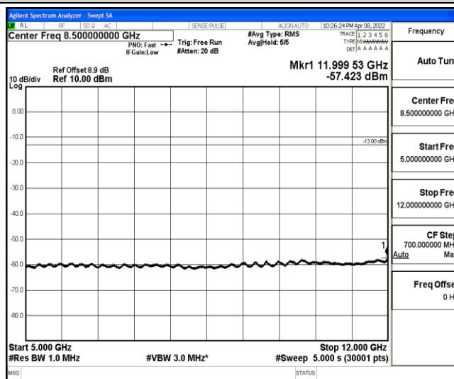
Band2-5MHz-QPSK-19175-1-0-High-5000-12000--57.42-PASS
