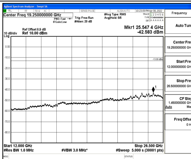
Band2-5MHz-QPSK-18900-1-0-Low-12000-26500--42.58-PASS
