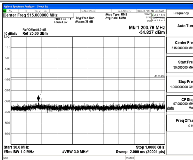
Band2-5MHz-16QAM-18900-1-0-Low-30-1000--34.83-PASS
