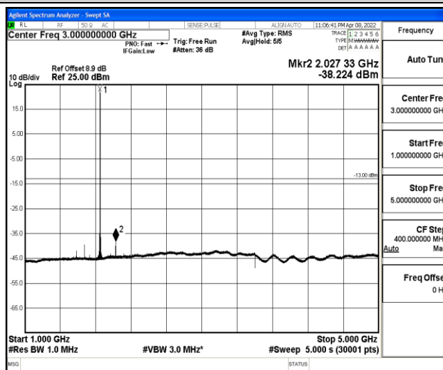
Band2-15MHz-QPSK-18675-1-0-Low-1000-5000--38.22-PASS
