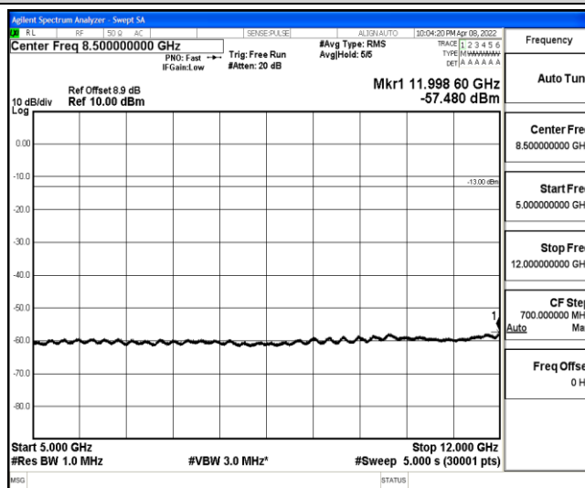
Band2-3MHz-16QAM-19185-1-0-High-5000-12000--57.48-PASS
