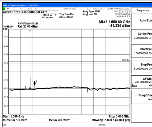
Band4-10MHz-QPSK-20000-1-0-Low-1000-5000--41.23-PASS
