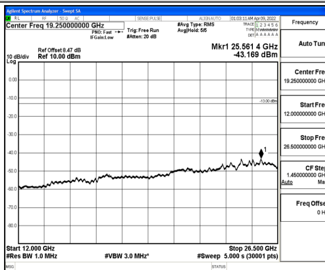
Band4-3MHz-QPSK-20175-1-0-Low-12000-26500--43.17-PASS
