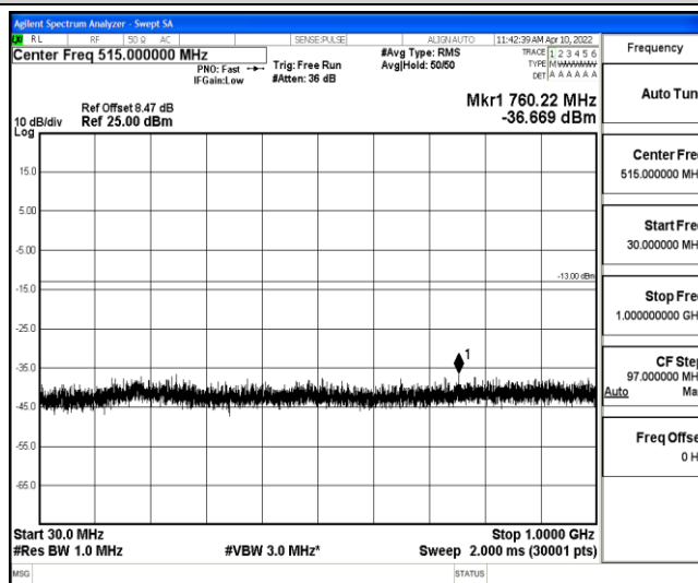
Band4-15MHz-QPSK-20175-1-0-Low-30-1000--36.67-PASS
