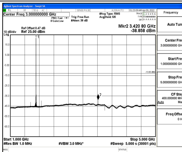
Band4-5MHz-16QAM-19975-1-0-Low-1000-5000--38.86-PASS
