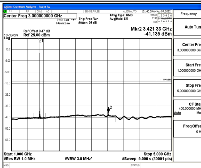
Band4-10MHz-16QAM-20000-1-0-Low-1000-5000--41.14-PASS
