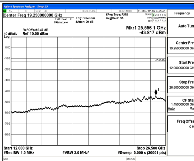
Band4-15MHz-QPSK-20175-1-0-Low-12000-26500--43.82-PASS
