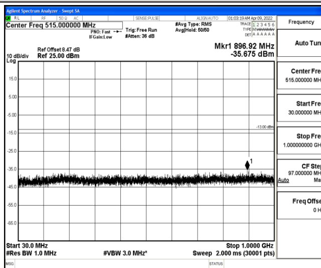
Band4-3MHz-16QAM-20175-1-0-Low-30-1000--35.68-PASS
