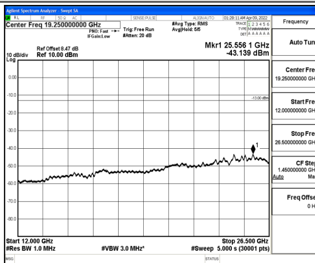
Band4-5MHz-16QAM-20175-1-0-Low-12000-26500--43.14-PASS
