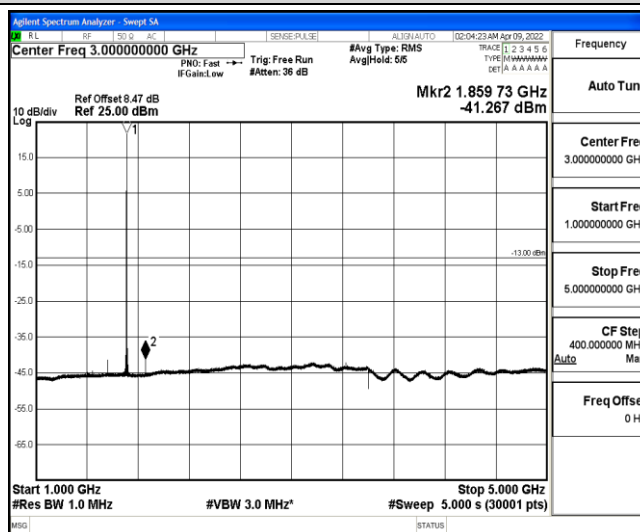
Band4-15MHz-QPSK-20025-1-0-Low-1000-5000--41.27-PASS
