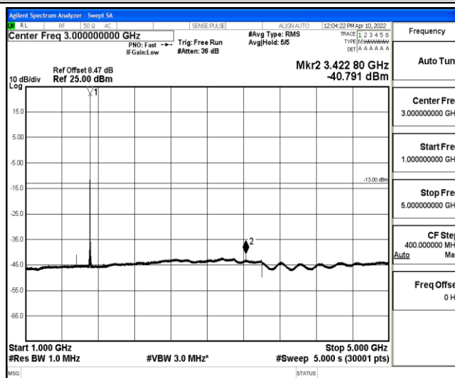
Band4-20MHz-16QAM-20050-1-0-Low-1000-5000--40.79-PASS
