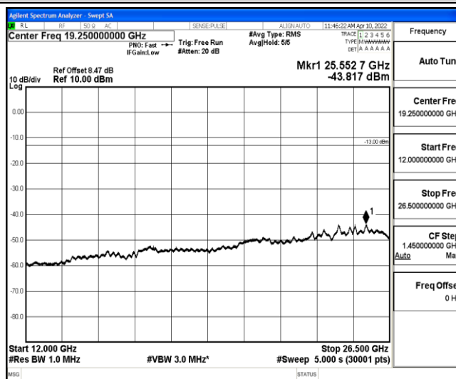
Band4-15MHz-16QAM-20175-1-0-Low-12000-26500--43.82-PASS
