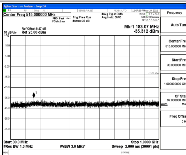
Band4-20MHz-16QAM-20175-1-0-Low-30-1000--35.31-PASS
