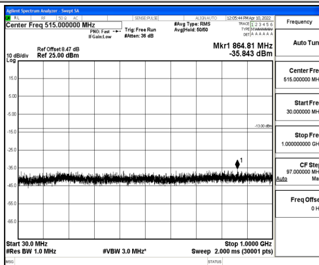
Band4-20MHz-QPSK-20175-1-0-Low-30-1000--35.84-PASS
